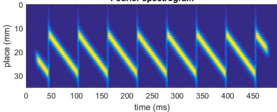
Fourier spectrogram
