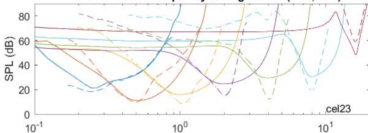
neural threshold frequency-tuning curves (EPL,man)
