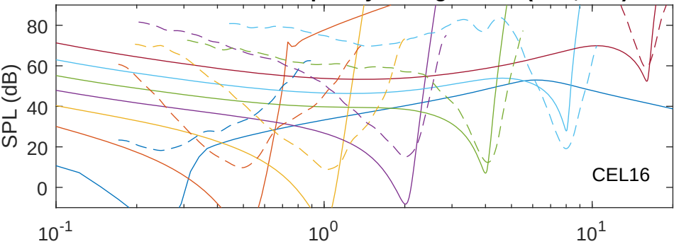
neural threshold frequency-tuning curves (EPL,man)
