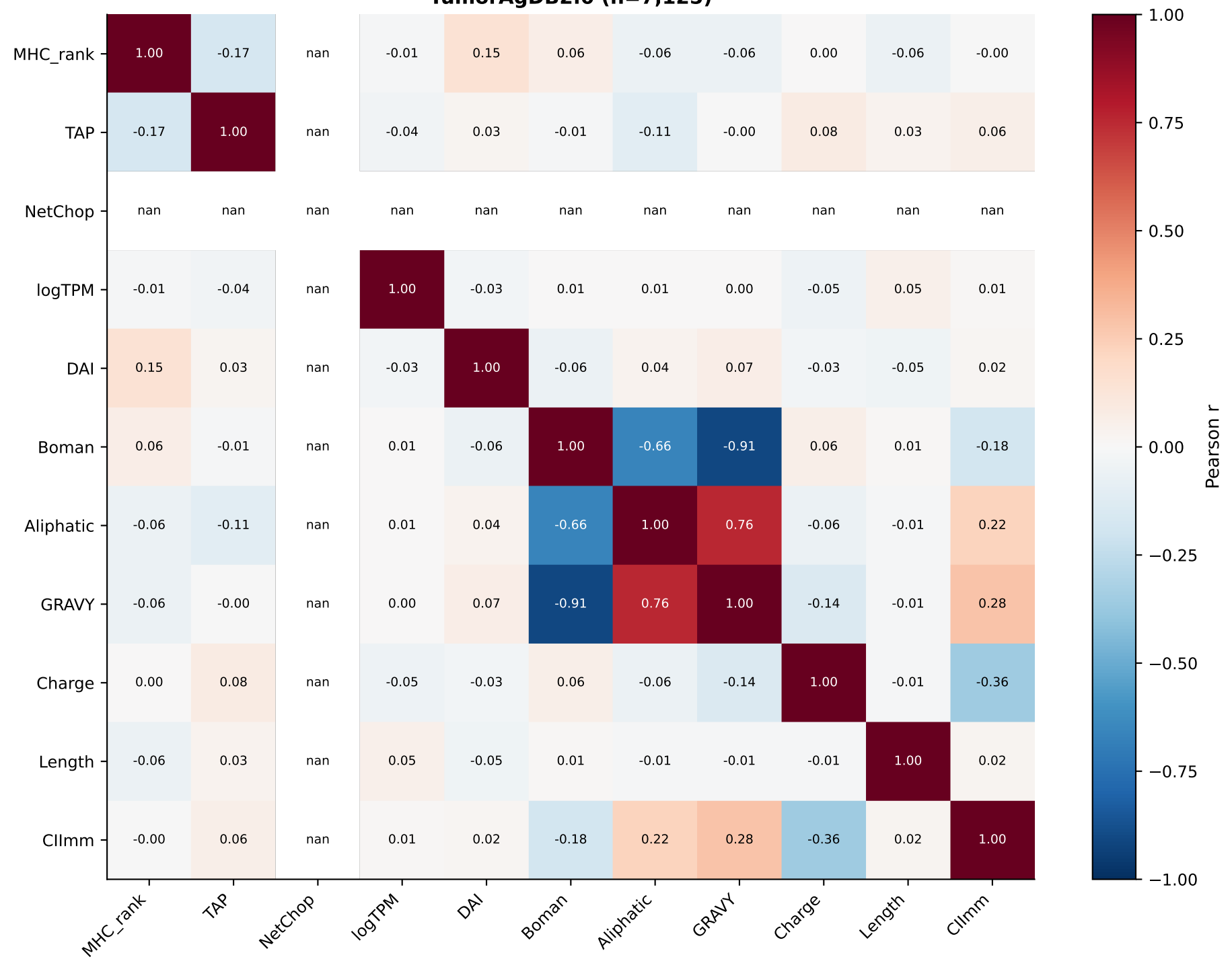
Supplementary Figure S2. FiLM Feature Correlation Matrix TumorAgDB2.0 (n=7,125)
