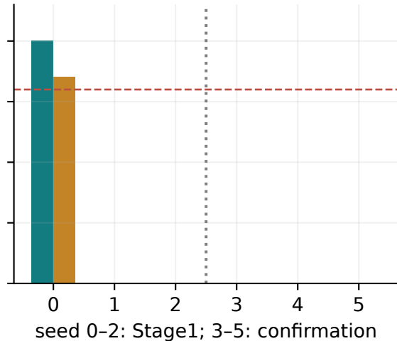
SAC-off · warmup5000
