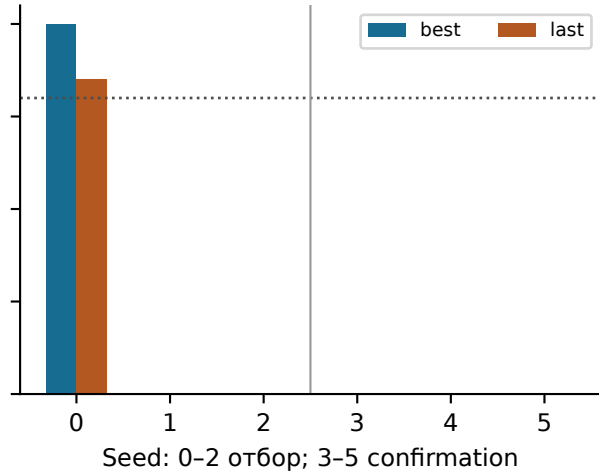
SAC-off, warmup5000
