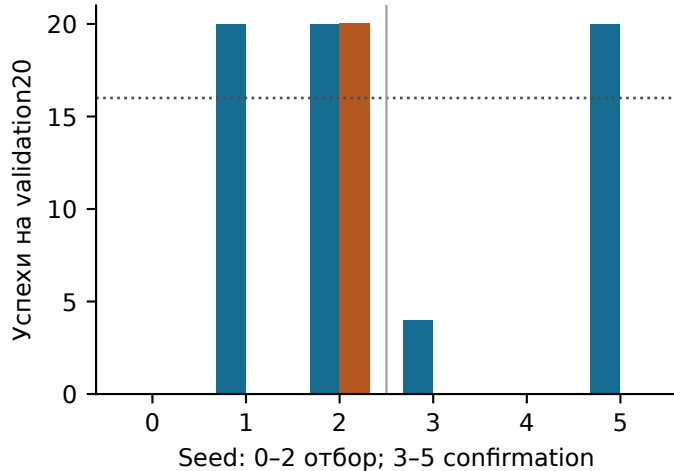
DDPG-on, warmup5000
