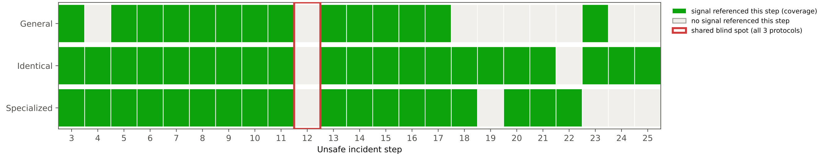
Current-step signal coverage on unsafe steps (shared blind spots outlined)
