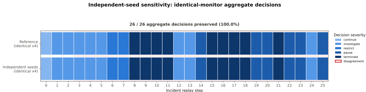
Figure 3: Independent-seed robustness of the identical-monitor ensemble. Removing the seed coupling with the general monitor left all 26 aggregate containment decisions unchanged (100.0% agreement) relative to the reference run, while the underlying category-step signal evidence changed (74 shared, 15 reference-only, 14 independent-seed-only keys).
