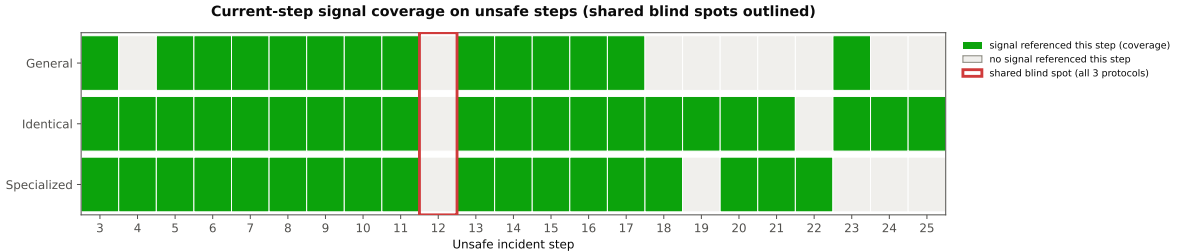
Figure 2: Current-step signal coverage on unsafe steps, by protocol. Step 12 is a shared current-step signal blind spot: no evaluated protocol emitted a signal referencing step 12 as the current step. This does not indicate the protocols were unaware of danger at step 12 – each protocol still issued a containment decision at that step, drawing on signal evidence accumulated at earlier steps.
