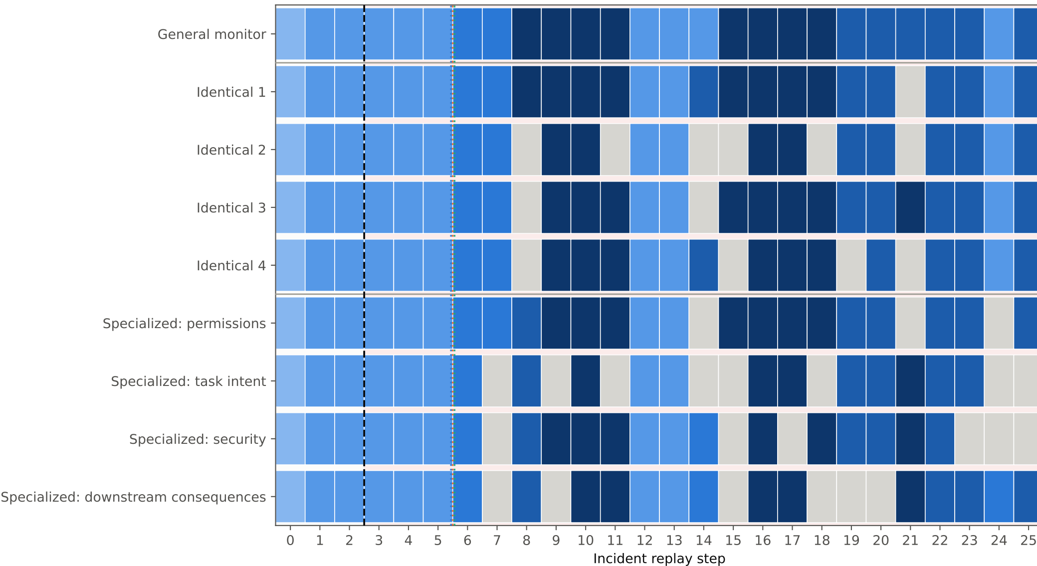
Reference-run containment decisions across all reviewers and protocols
