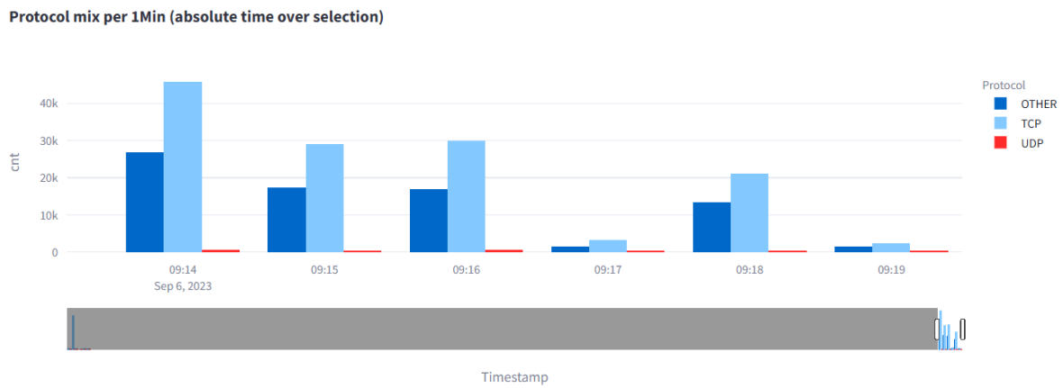
Figure 6.6: Dataset A (Real Network Environment Dataset): Instant messaging protocol mix per minute for 2023-09-06, zoom into time 09:14–09:19. UDP-dominated bursts could also indicate real-time interaction periods. A smaller increment than one minute would be needed to better recognize instant messaging.
