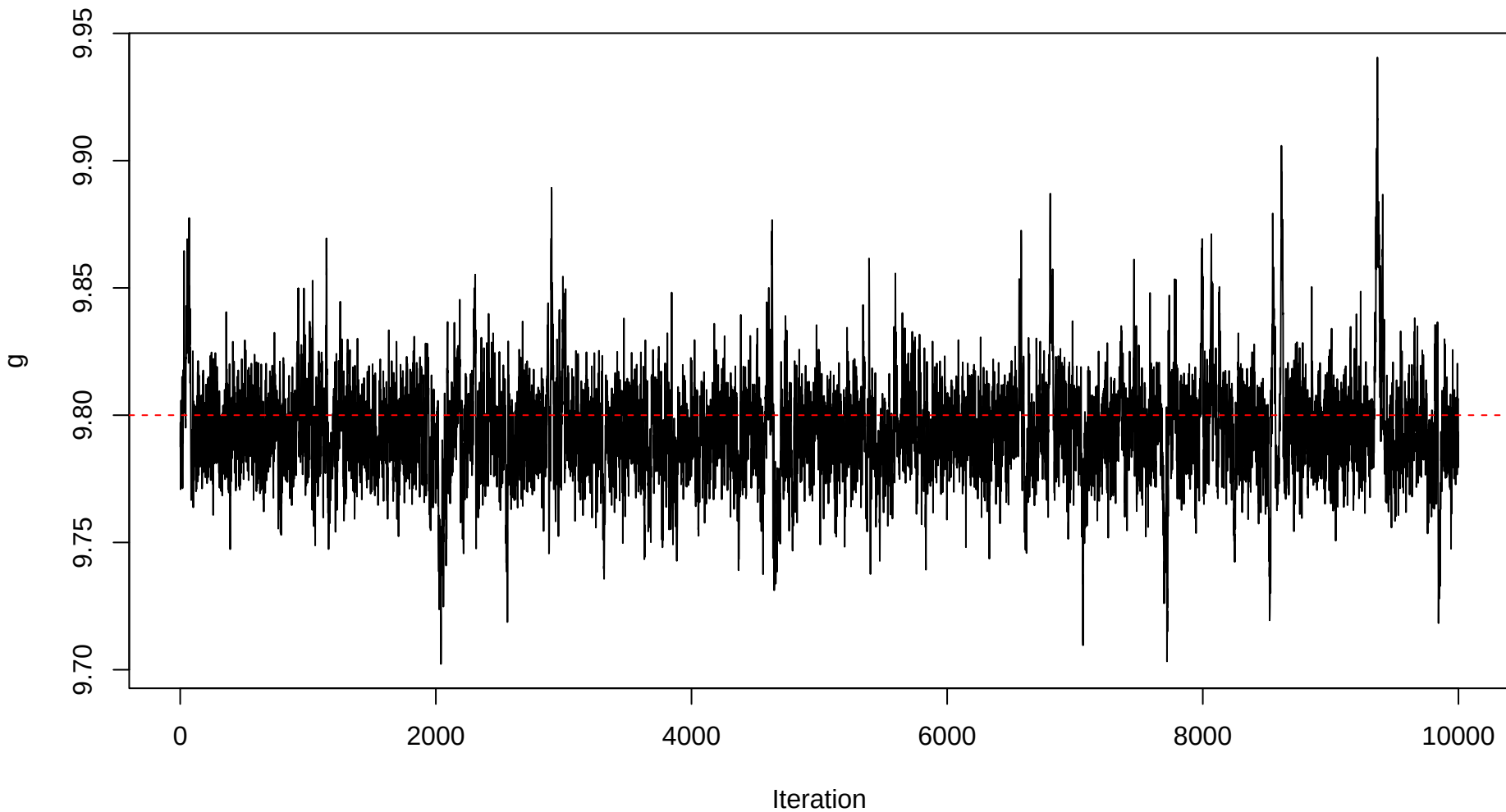
Trace plot – g – Sample 42
