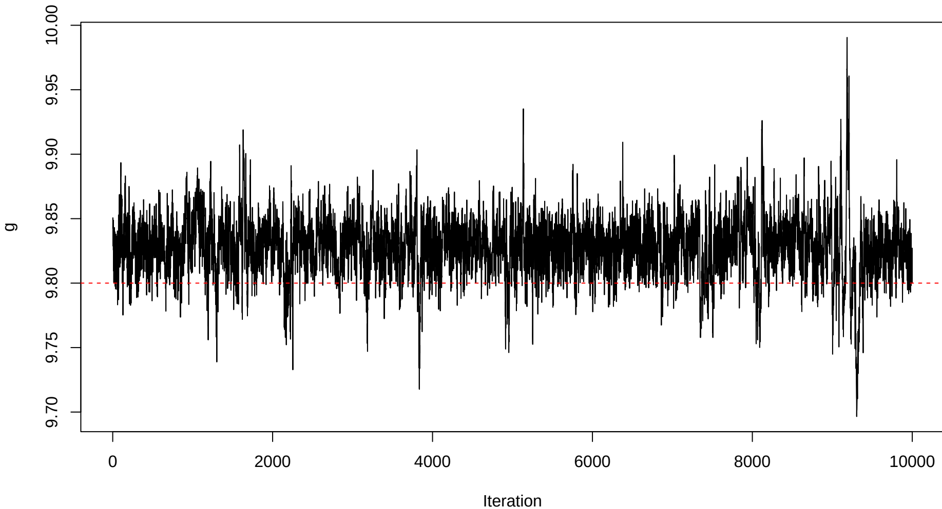
Trace plot – g – Sample 15
