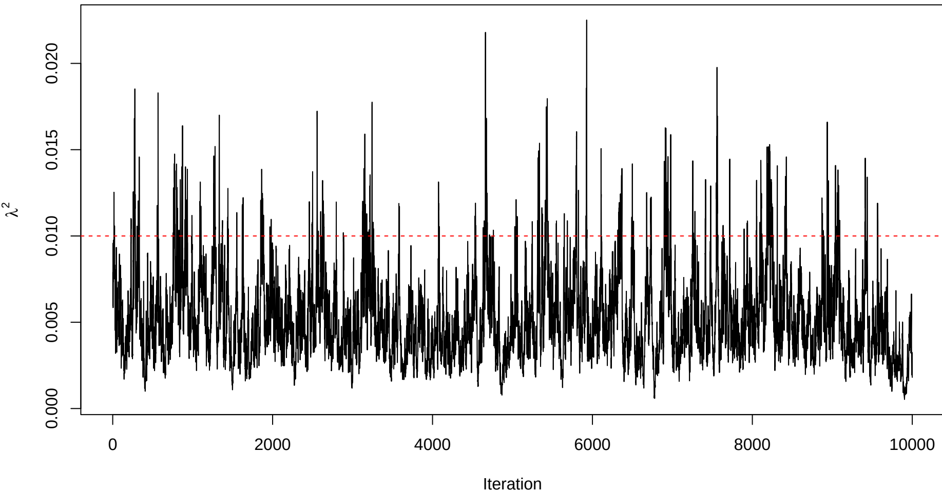
Trace plot – sigma_sq_err – Sample 7
