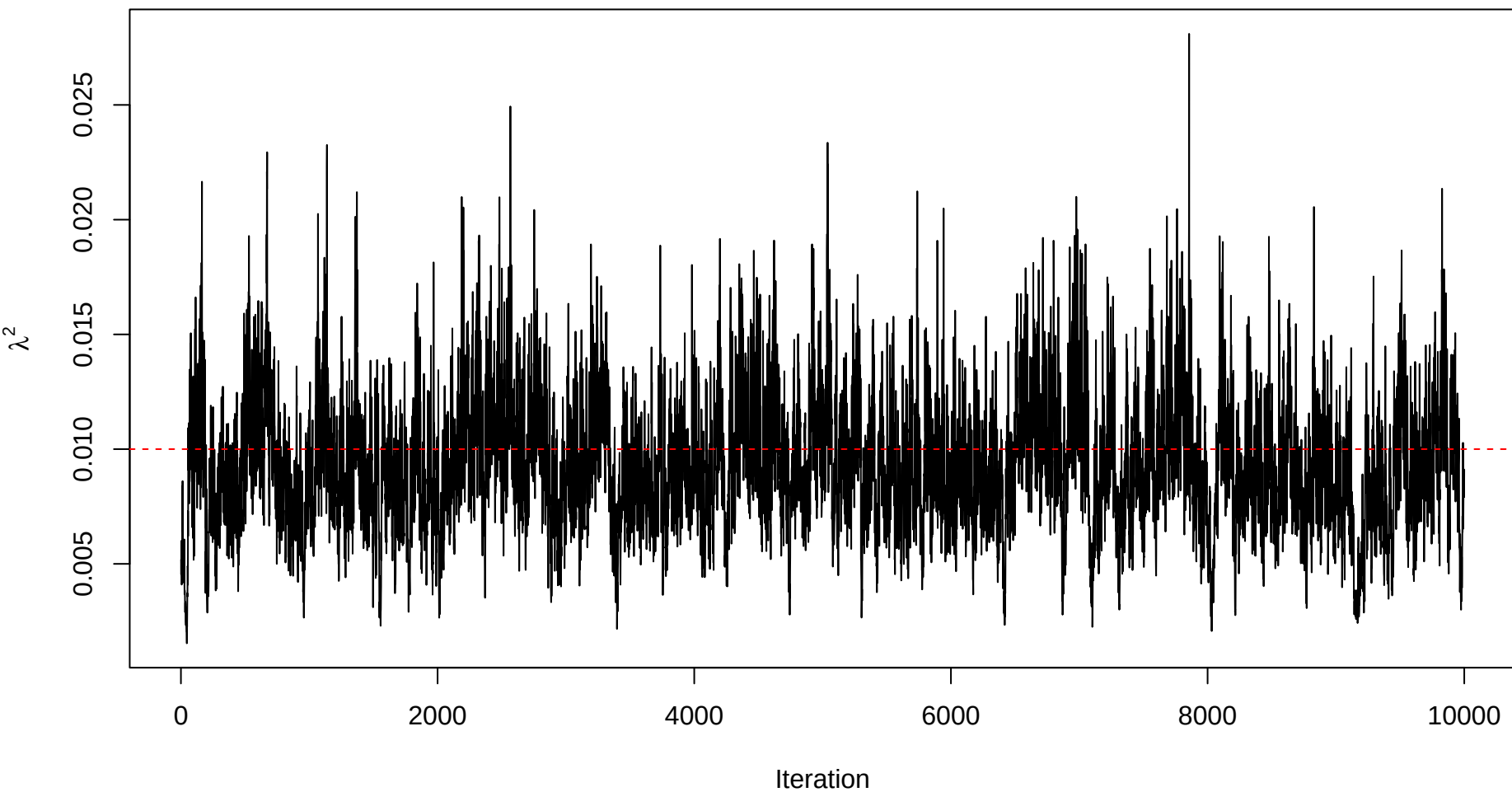
Trace plot – sigma_sq_err – Sample 37
