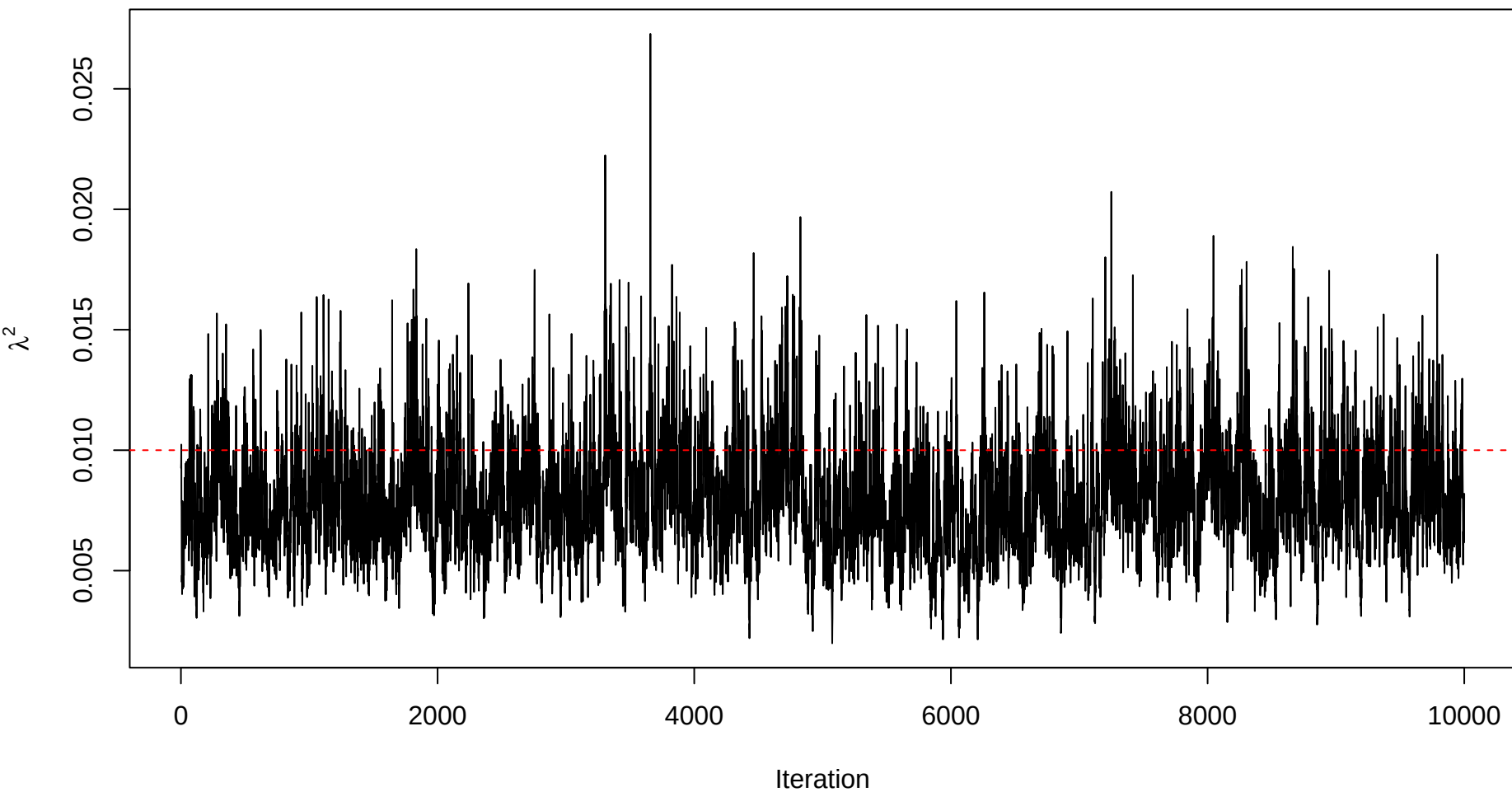
Trace plot – sigma_sq_err – Sample 35
