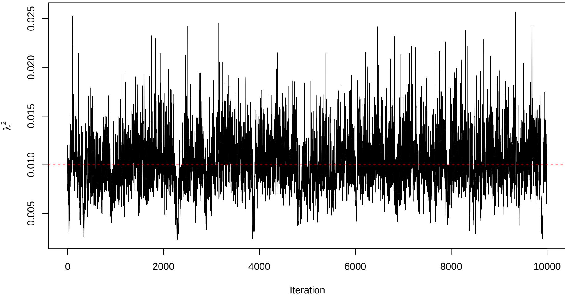
Trace plot – sigma_sq_err – Sample 33
