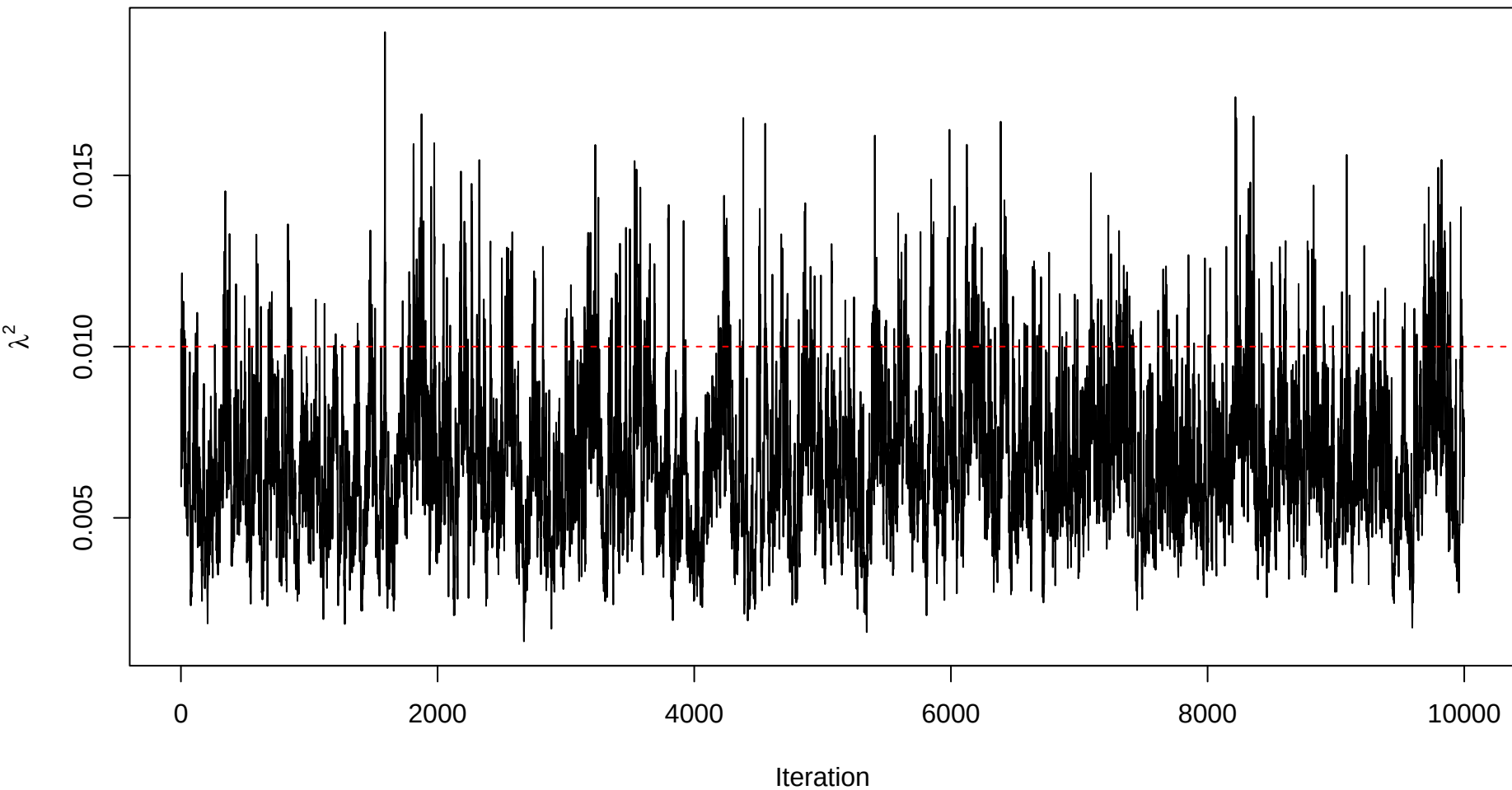
Trace plot – sigma_sq_err – Sample 14
