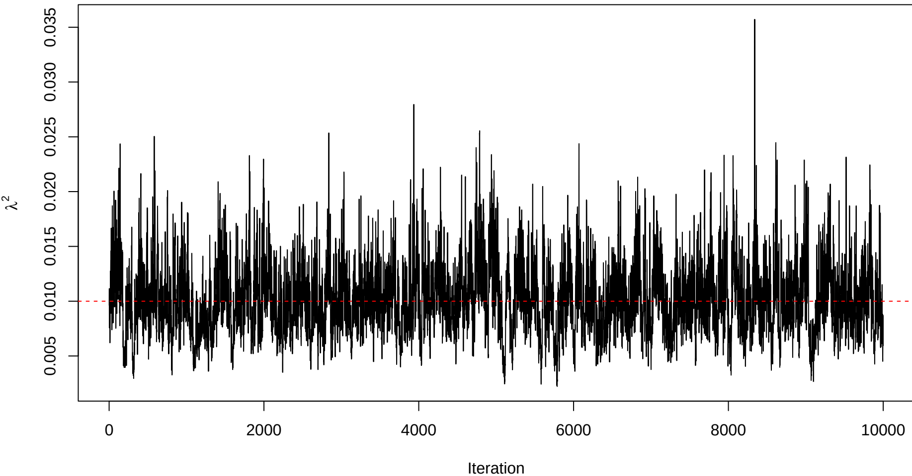
Trace plot – sigma_sq_err – Sample 10
