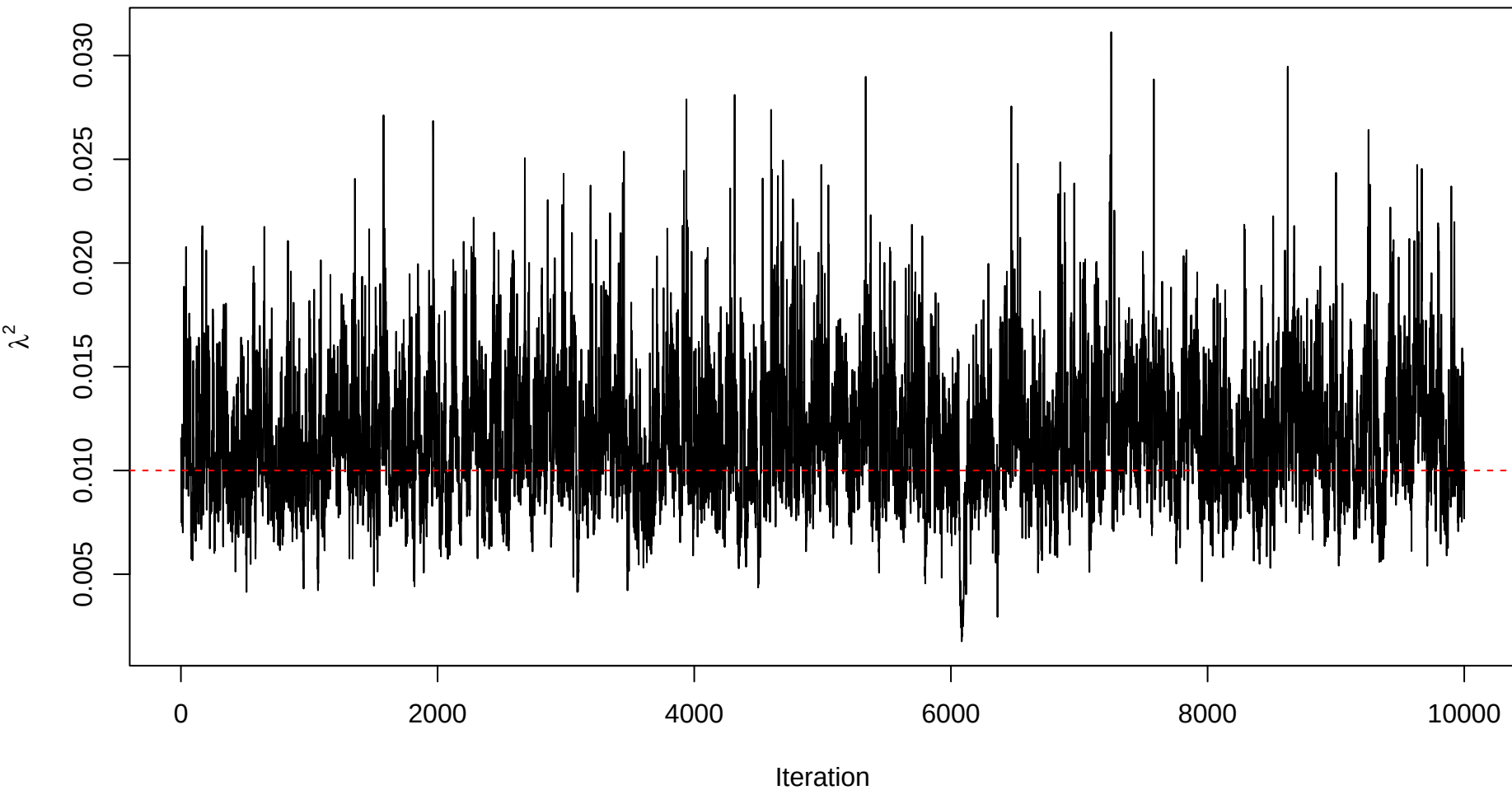
Trace plot – sigma_sq_err – Sample 19
