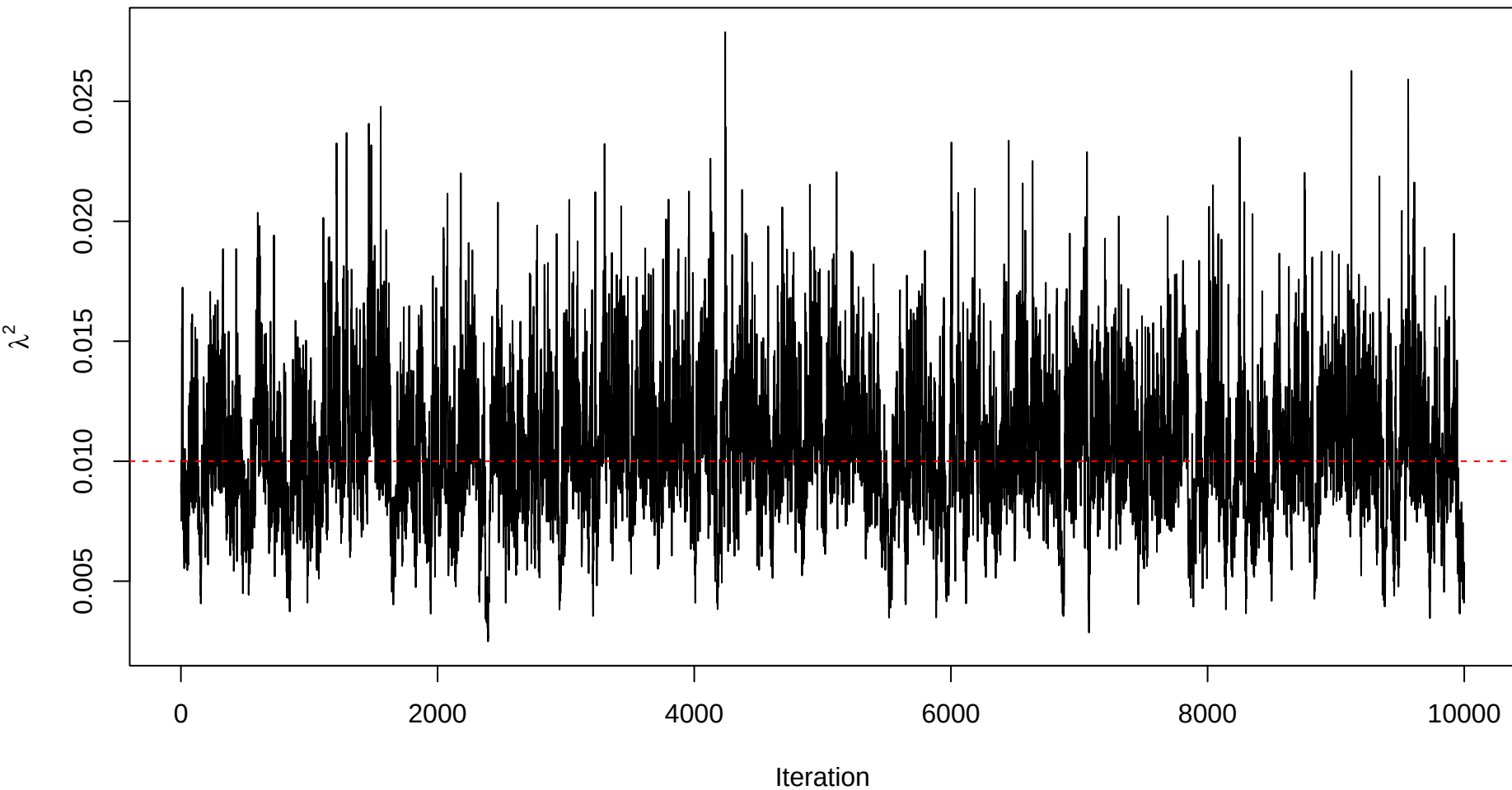
Trace plot – sigma_sq_err – Sample 1
