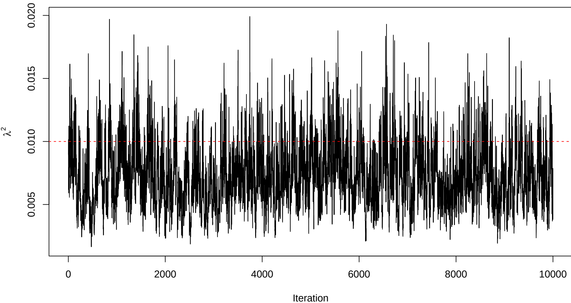
Trace plot – sigma_sq_err – Sample 5
