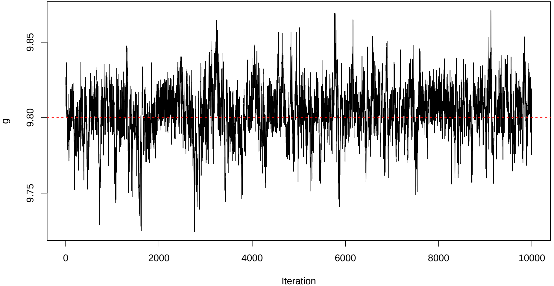
Trace plot – g – Sample 48
