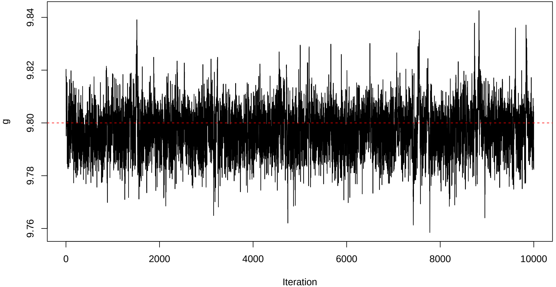
Trace plot – g – Sample 40
