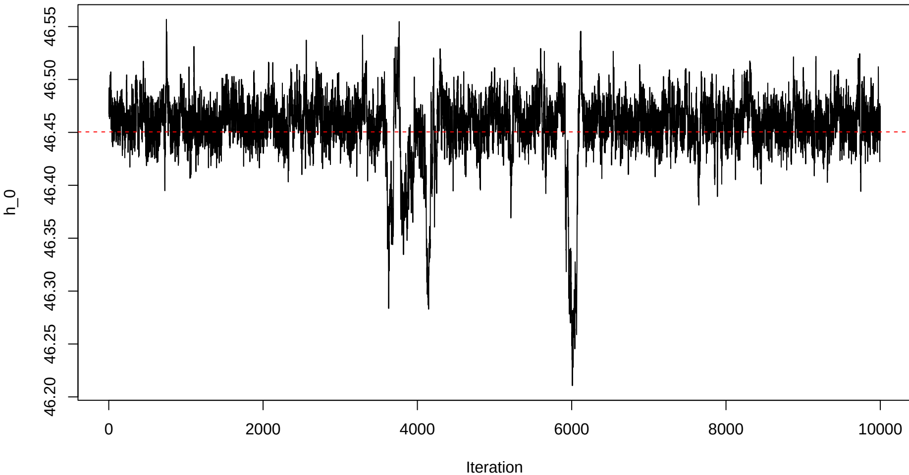
Trace plot – h0 – Sample 17
