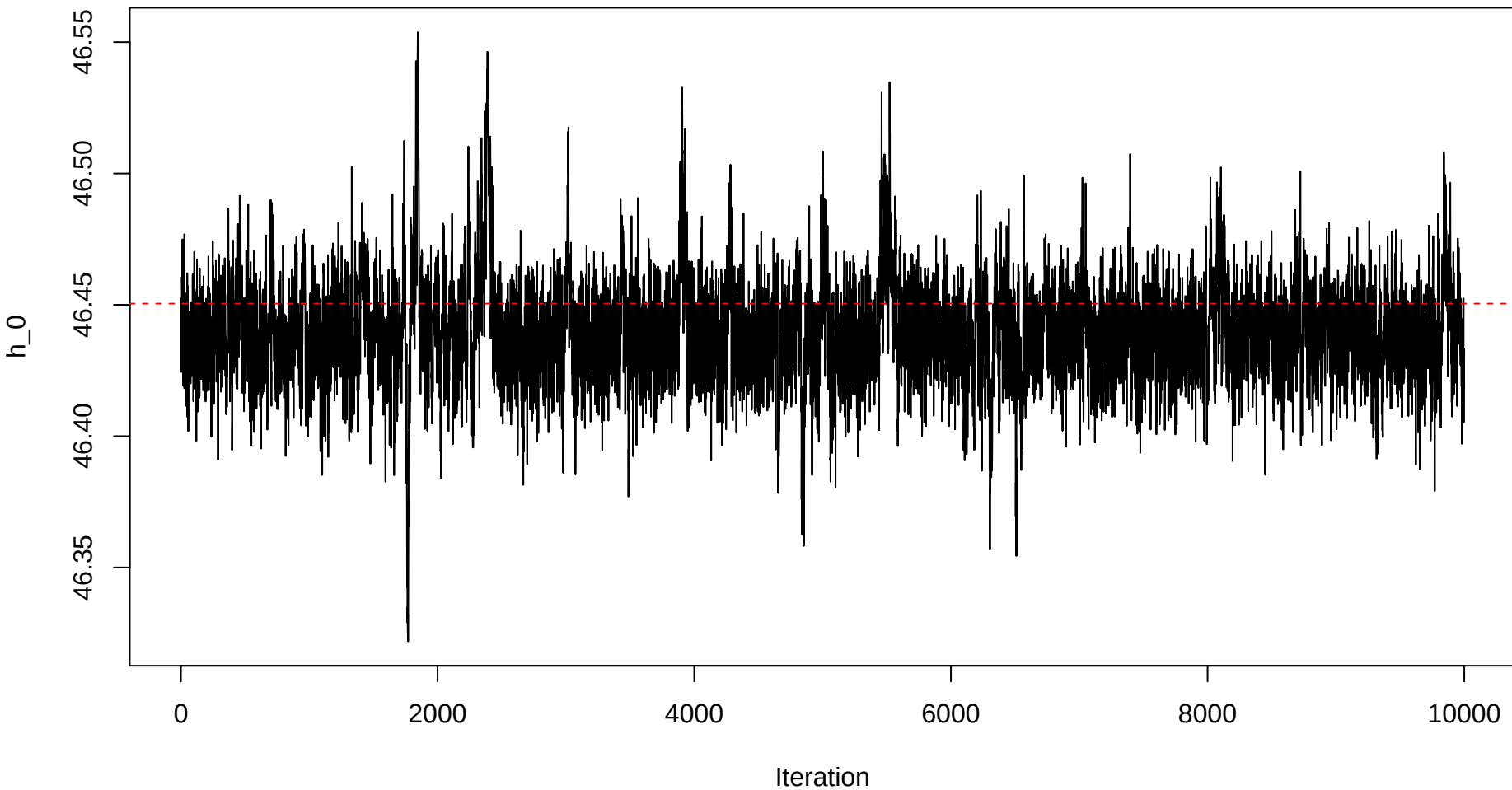
Trace plot – h0 – Sample 50
