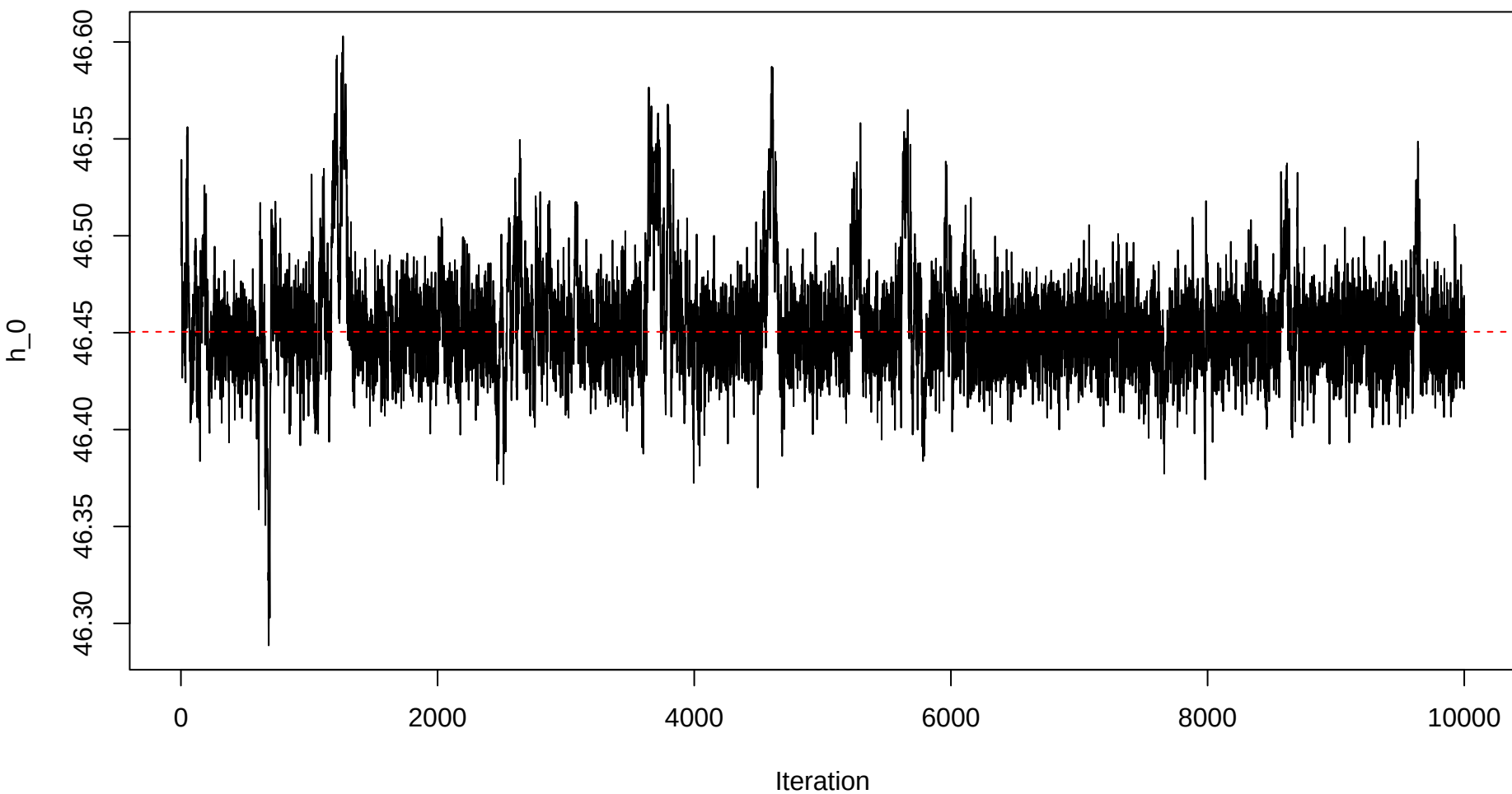
Trace plot – h0 – Sample 42
