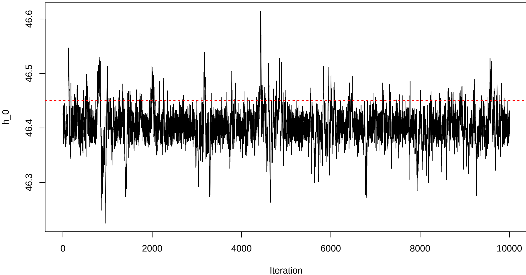
Trace plot – h0 – Sample 27
