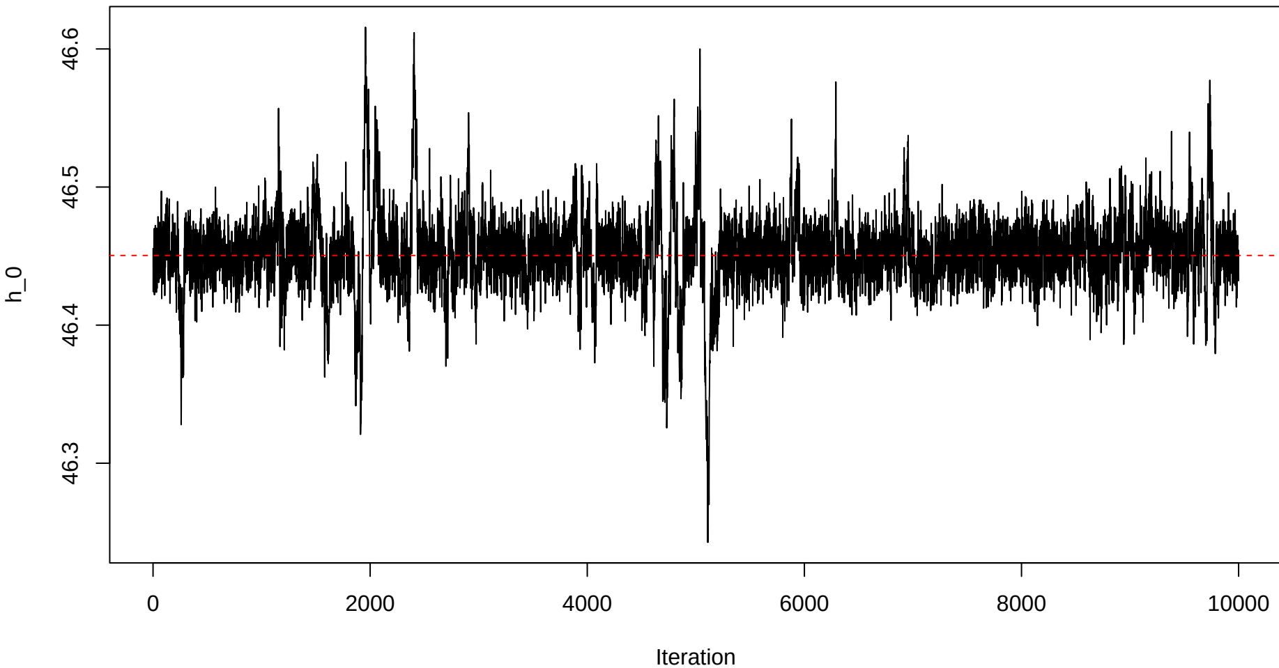
Trace plot – h0 – Sample 31
