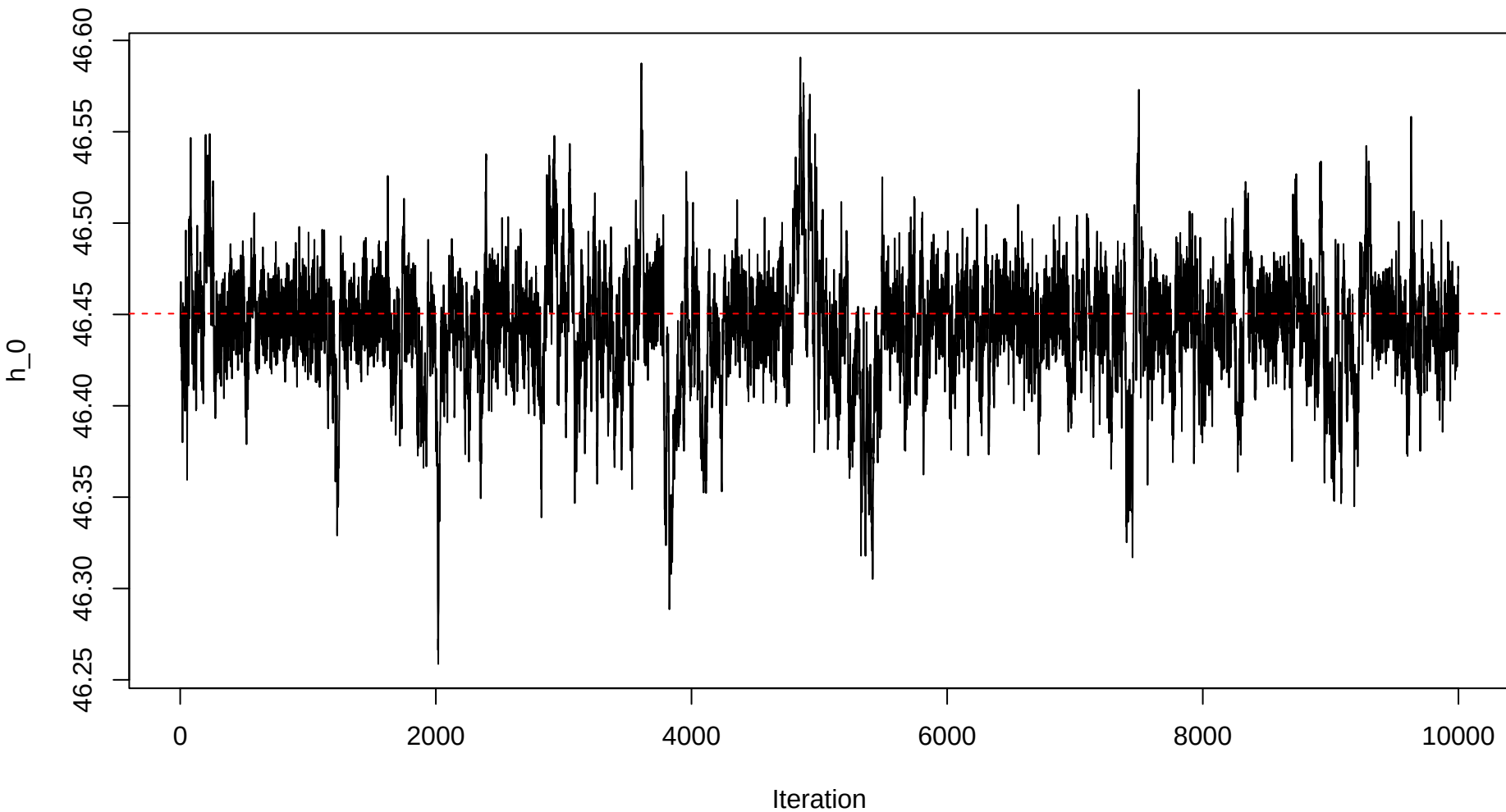
Trace plot – h0 – Sample 37
