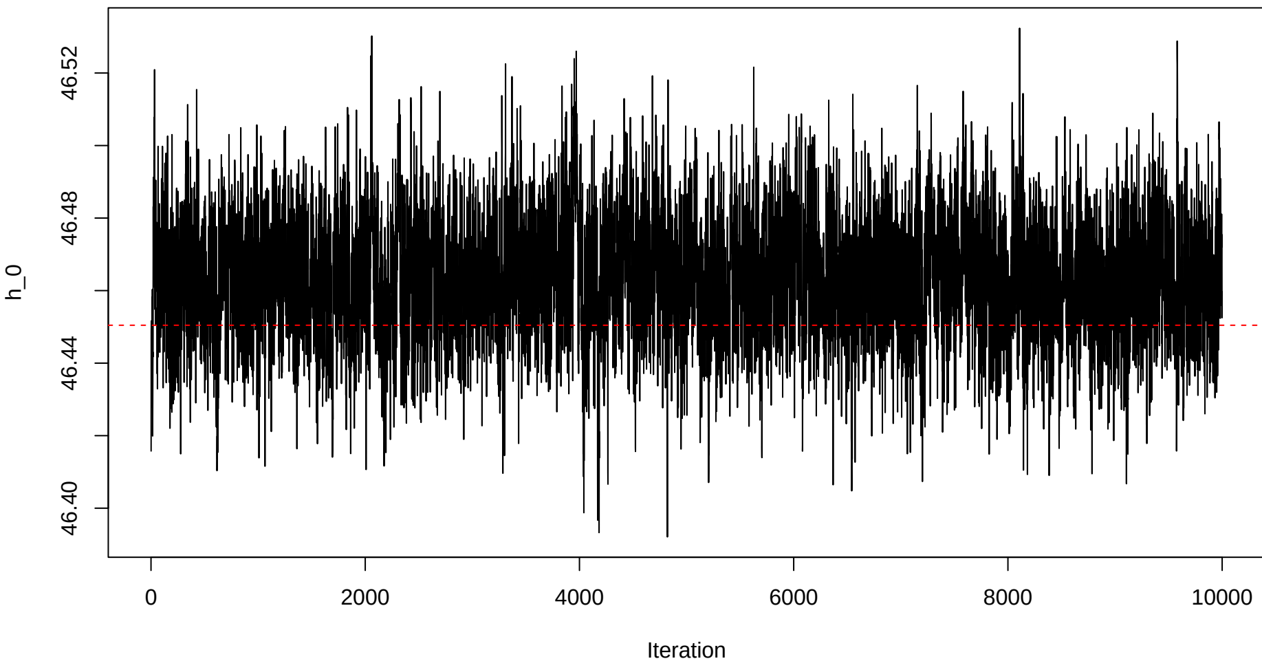
Trace plot – h0 – Sample 2
