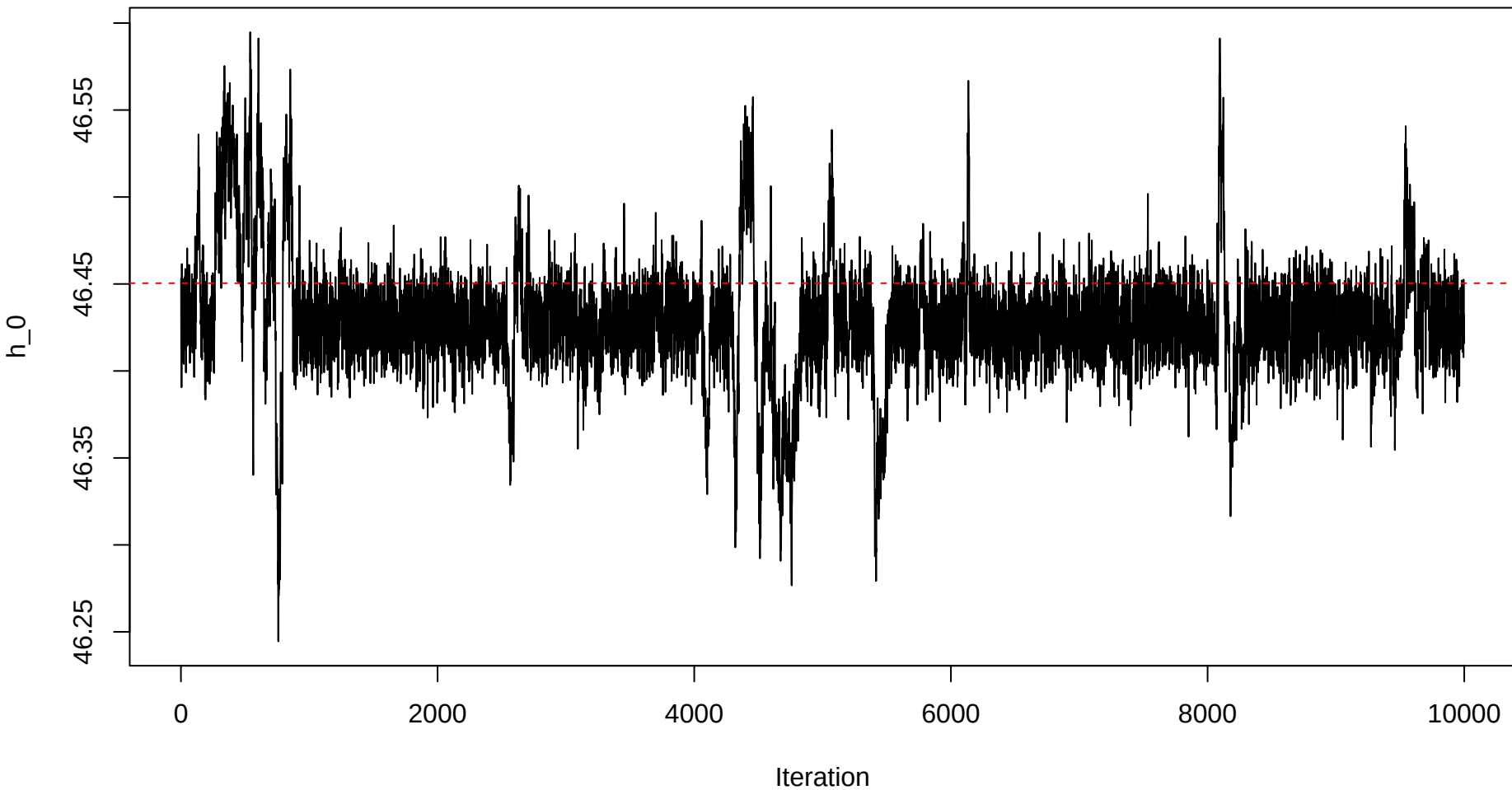
Trace plot – h0 – Sample 15
