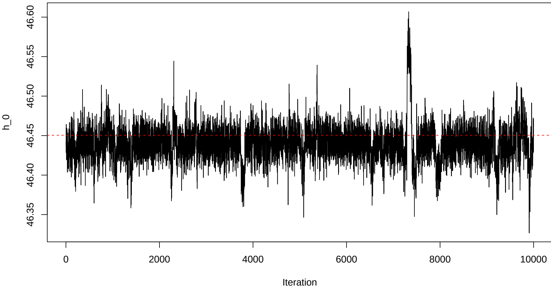
Trace plot – h0 – Sample 25
