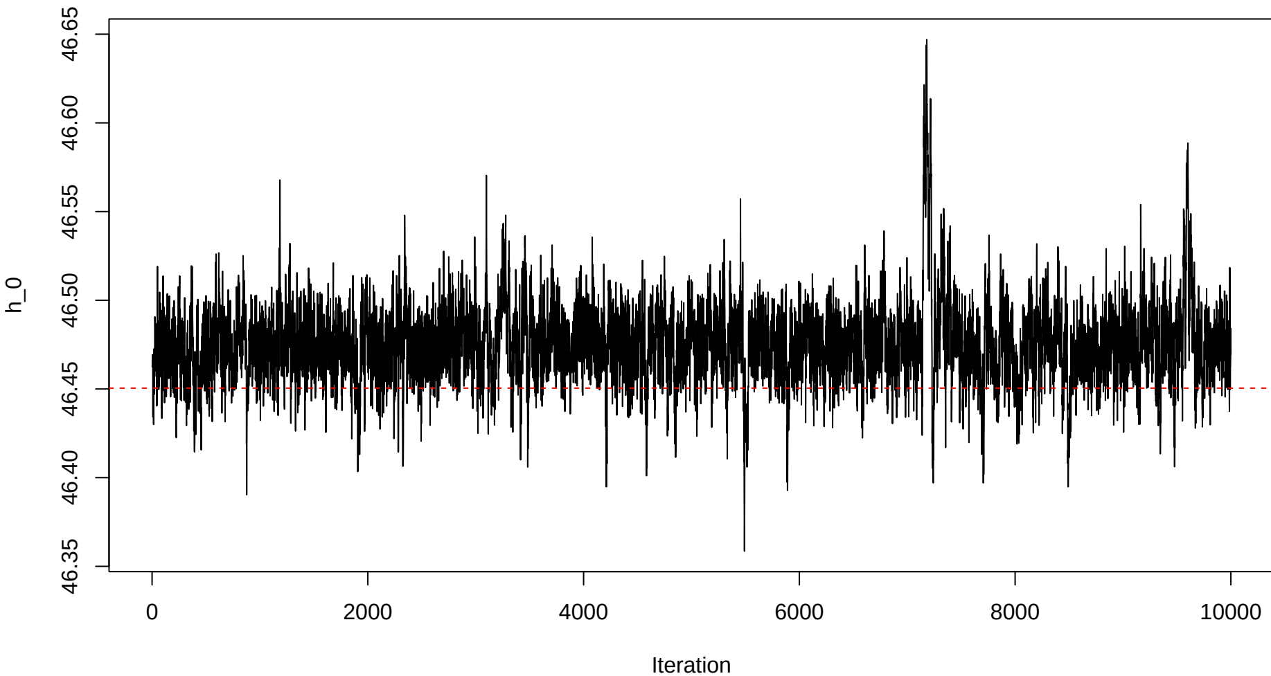
Trace plot – h0 – Sample 45
