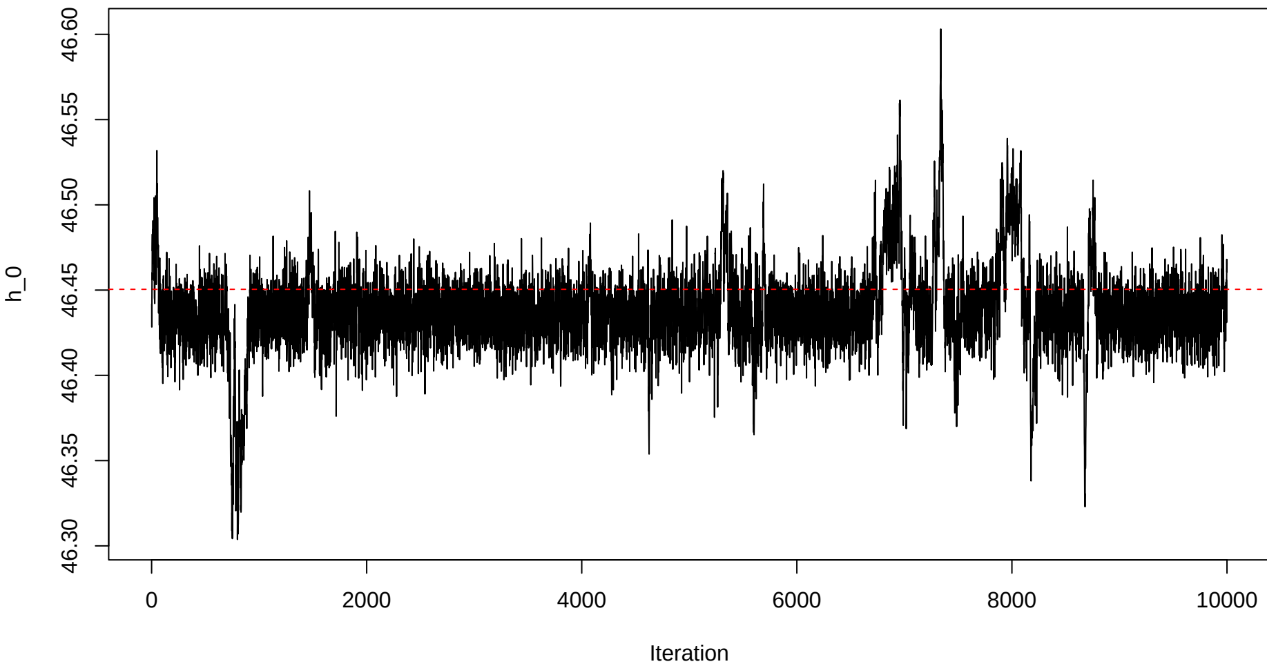
Trace plot – h0 – Sample 12
