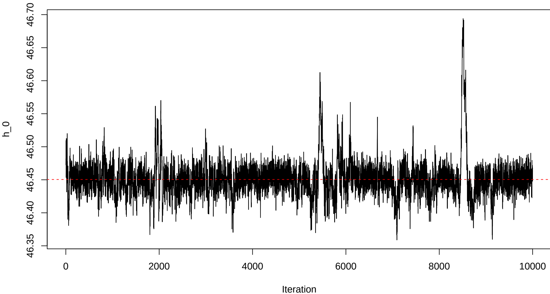
Trace plot – h0 – Sample 41
