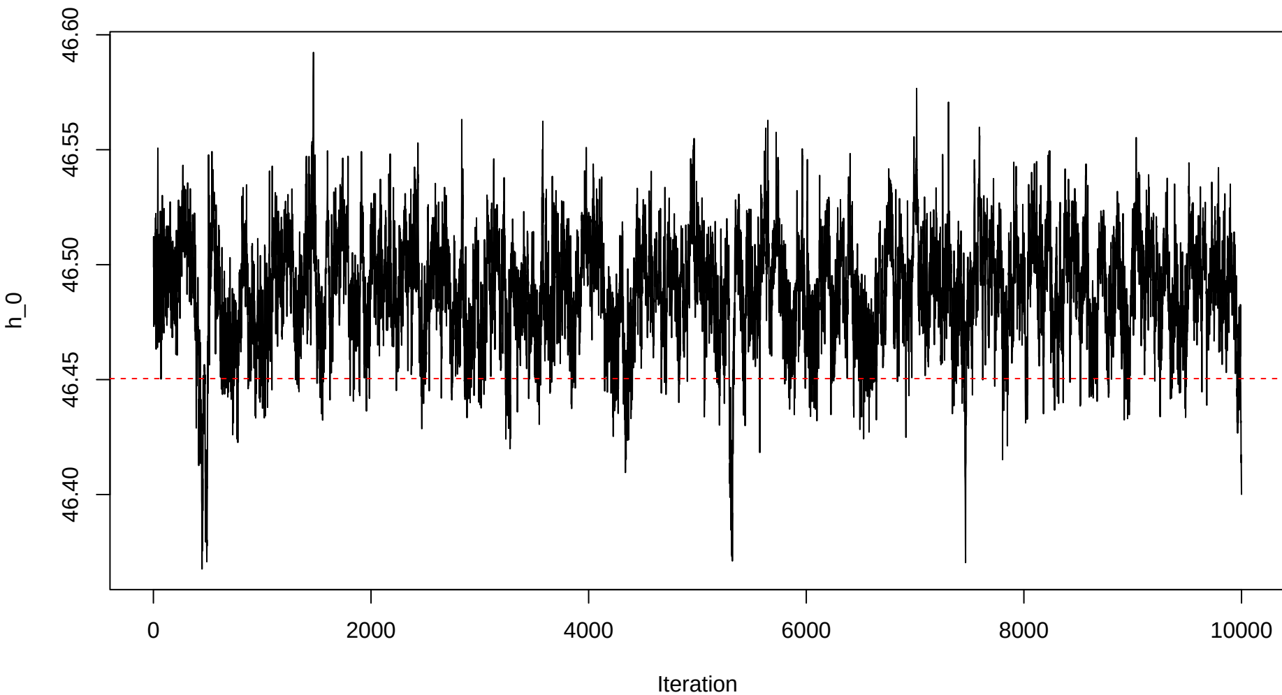
Trace plot – h0 – Sample 14
