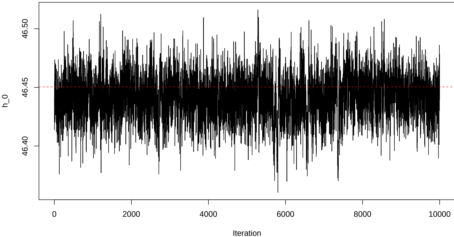
Trace plot – h0 – Sample 10
