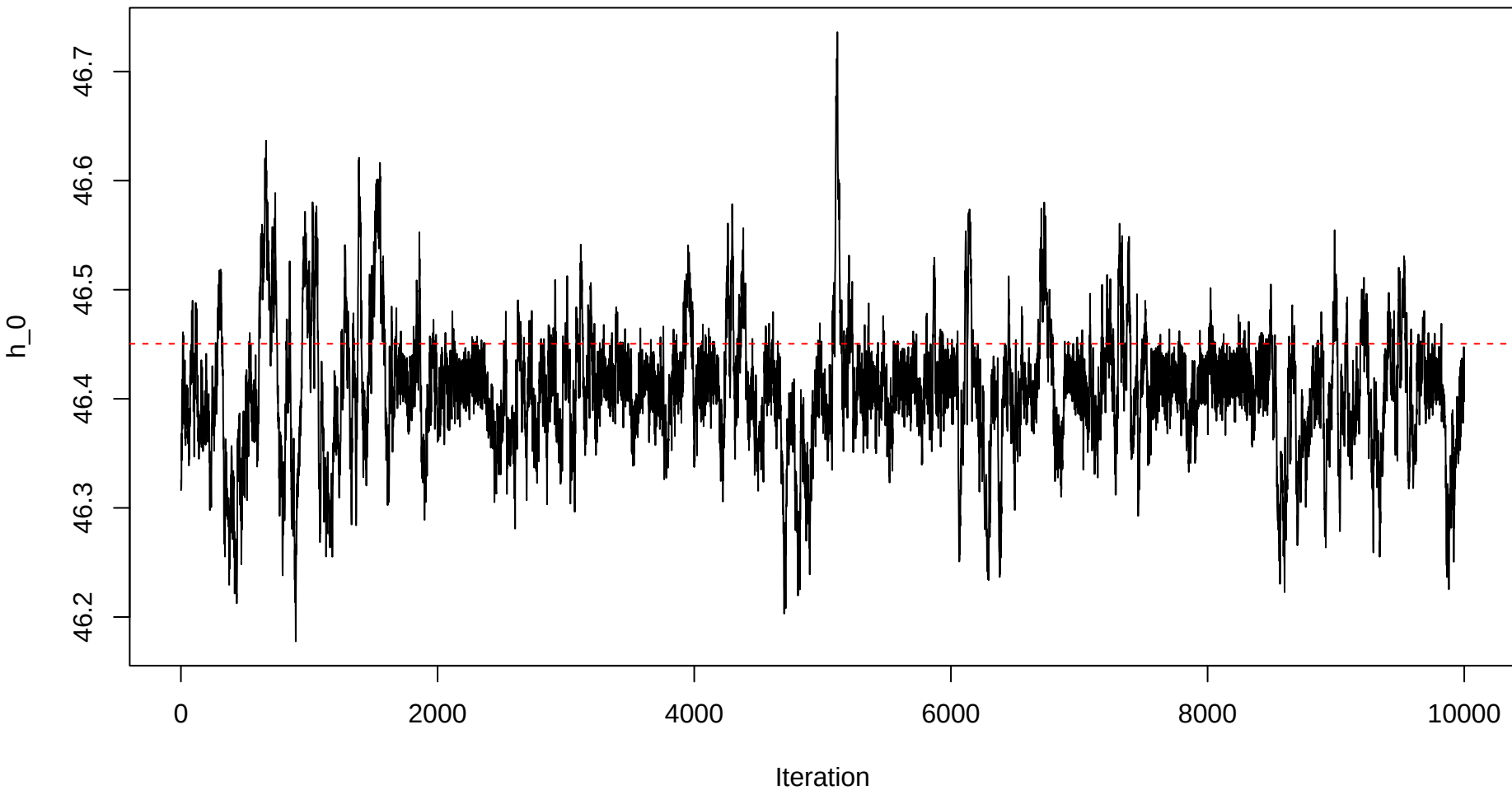
Trace plot – h0 – Sample 46
