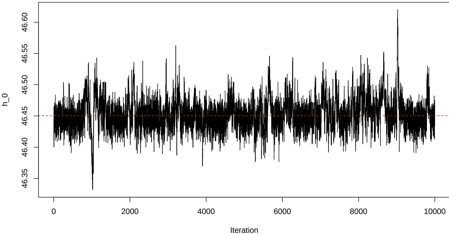
Trace plot – h0 – Sample 28
