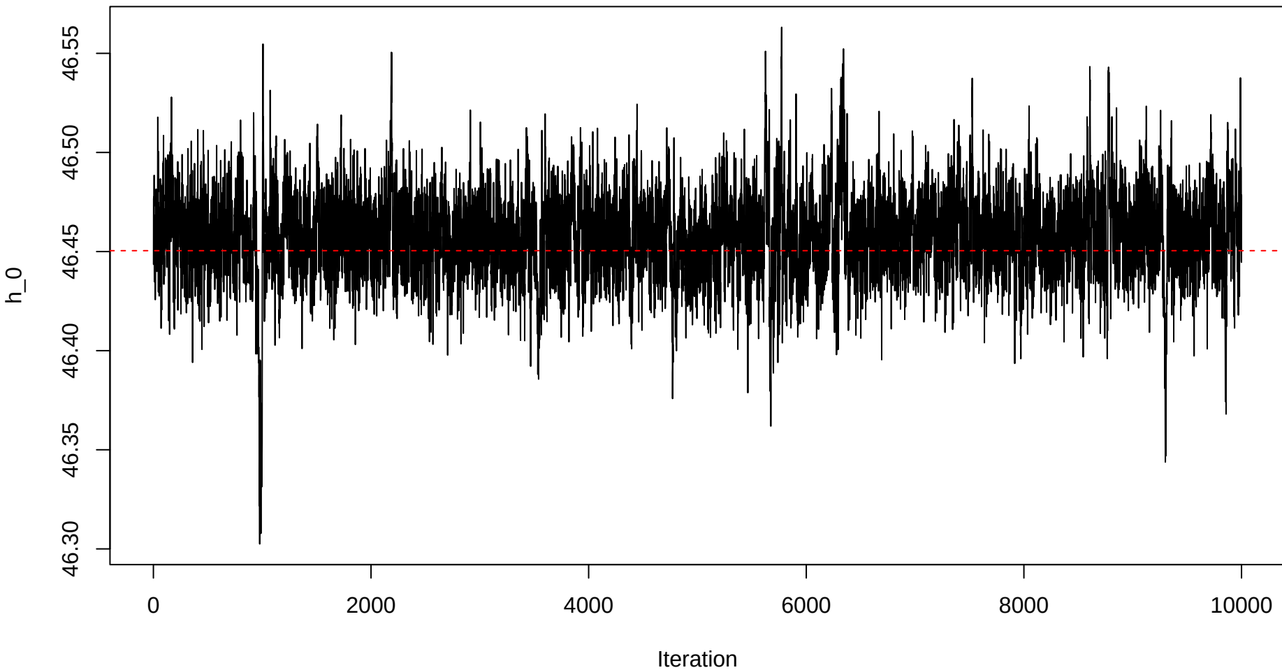
Trace plot – h0 – Sample 38
