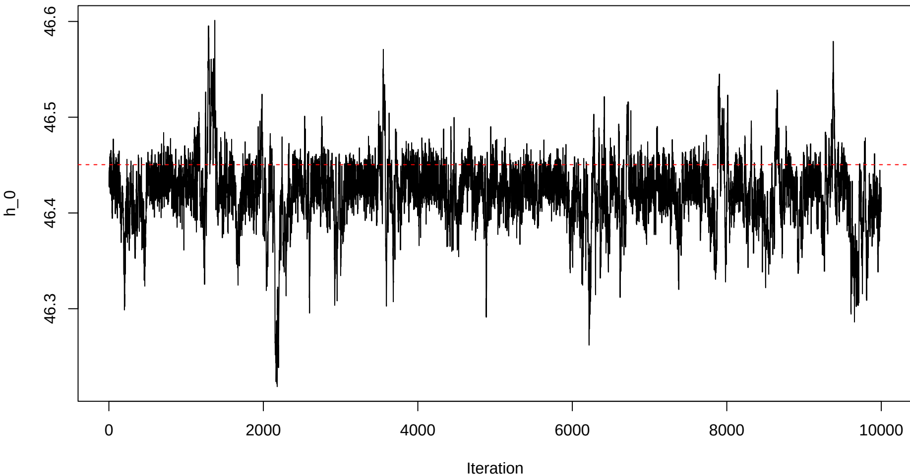
Trace plot – h0 – Sample 7
