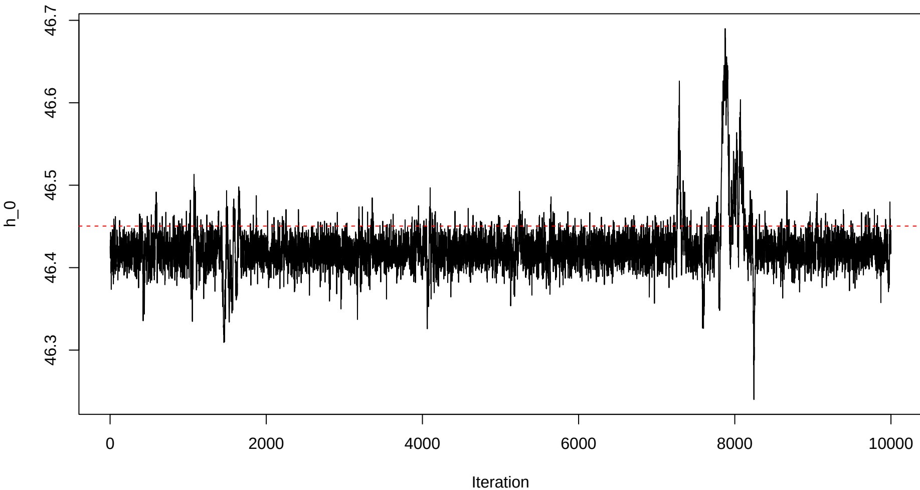
Trace plot – h0 – Sample 35
