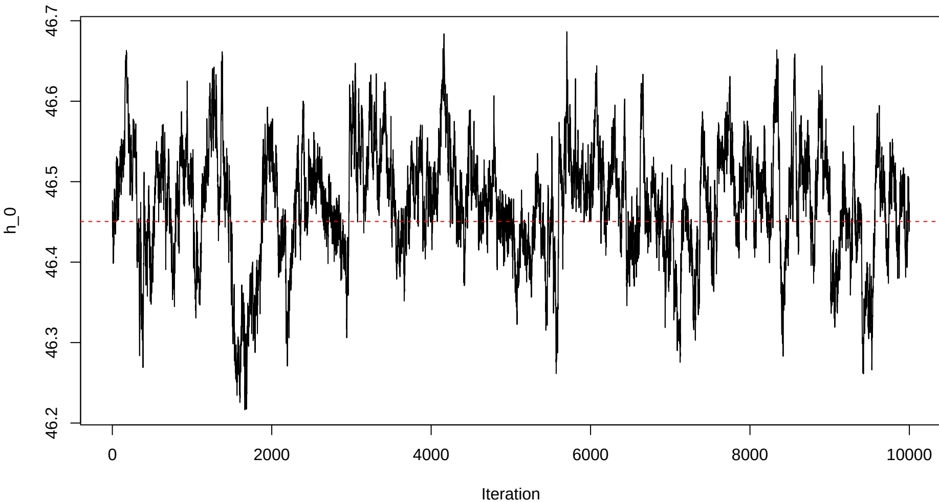
Trace plot – h0 – Sample 11
