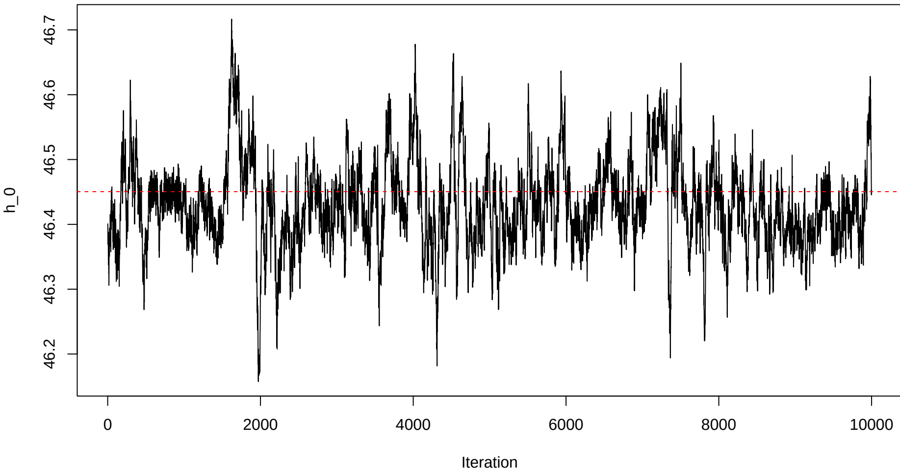
Trace plot – h0 – Sample 18
