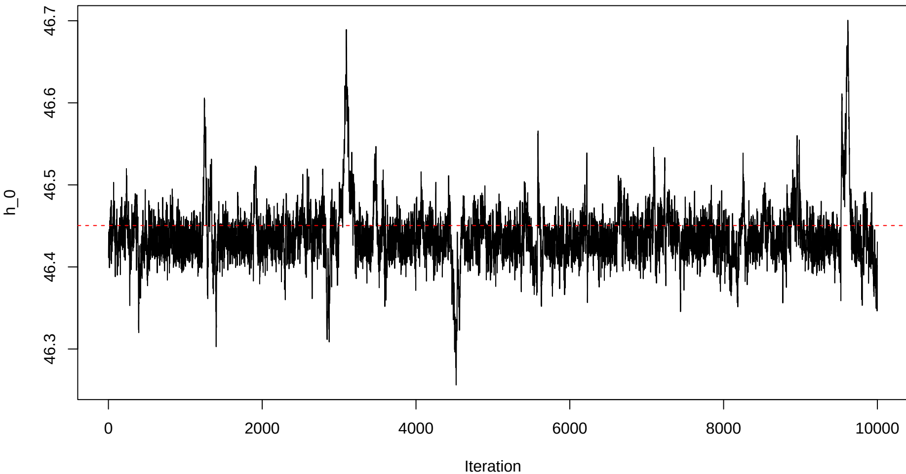
Trace plot – h0 – Sample 22
