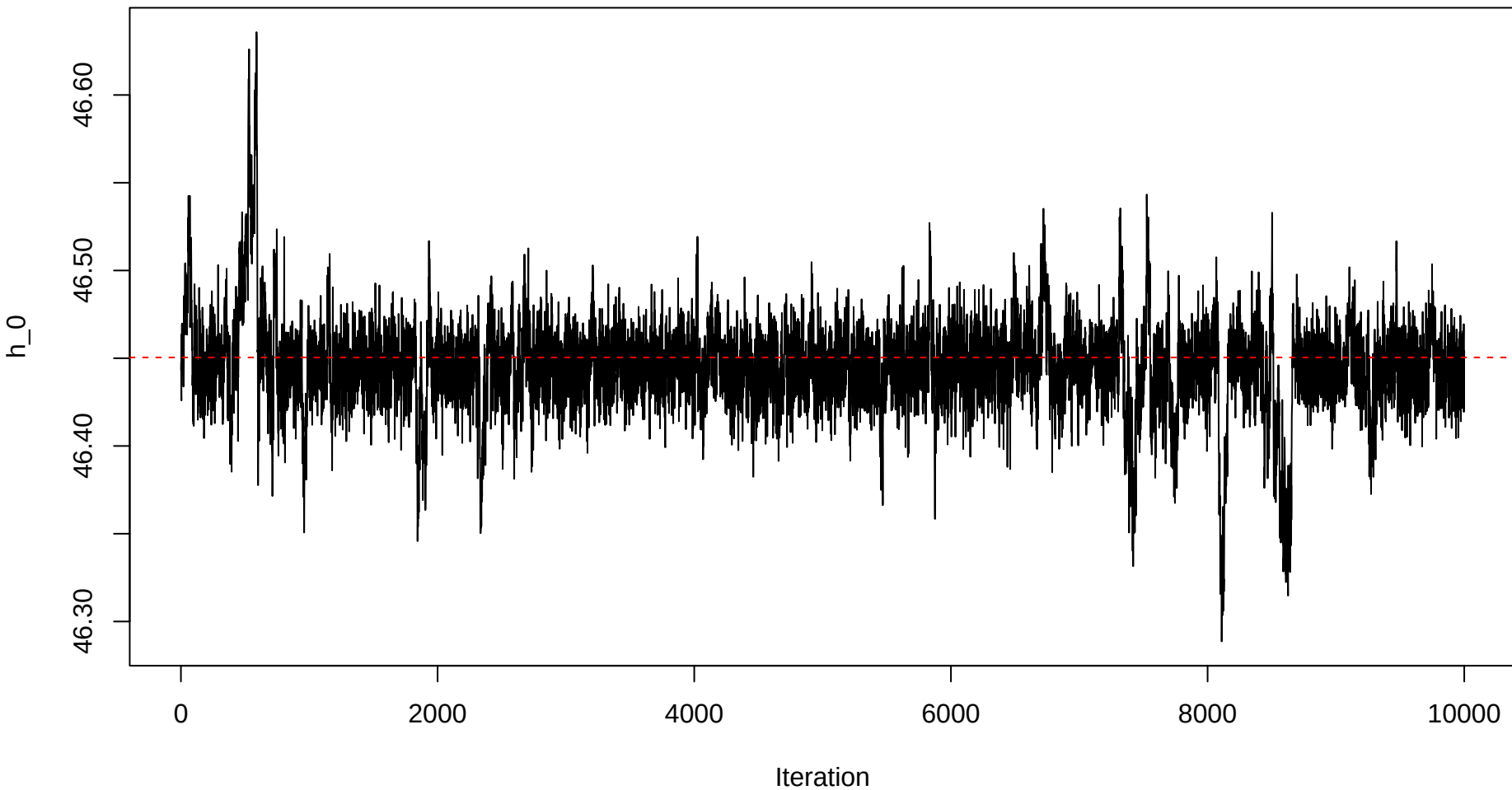
Trace plot – h0 – Sample 8
