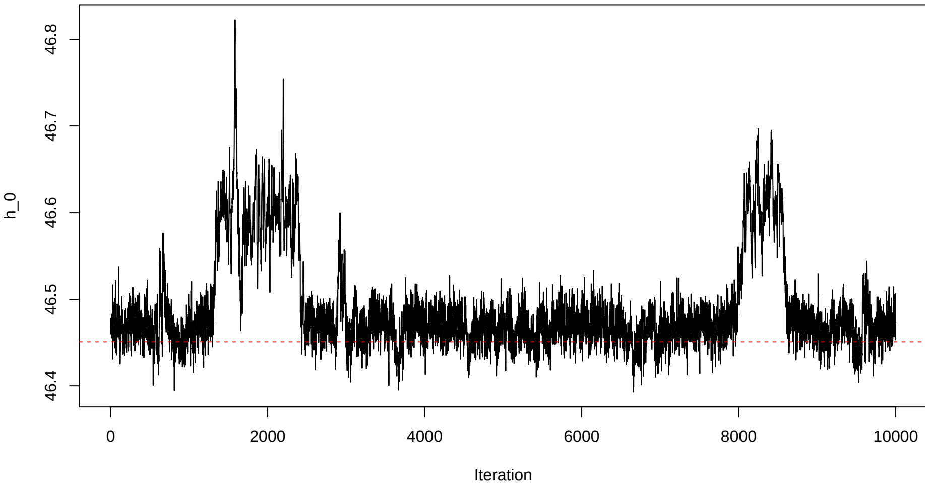
Trace plot – h0 – Sample 39
