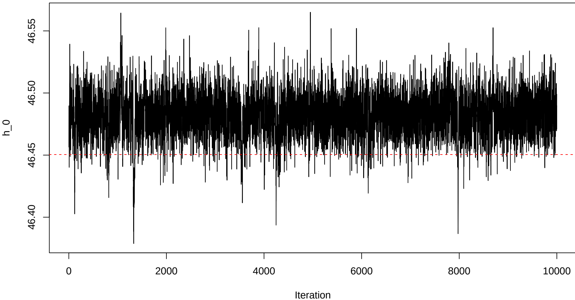
Trace plot – h0 – Sample 6
