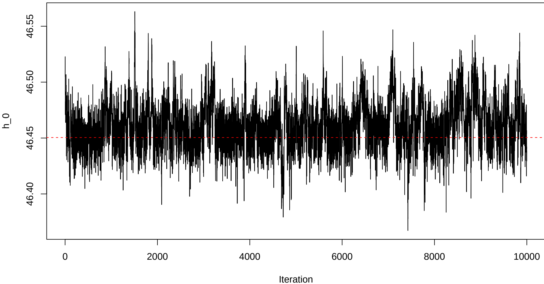
Trace plot – h0 – Sample 40
