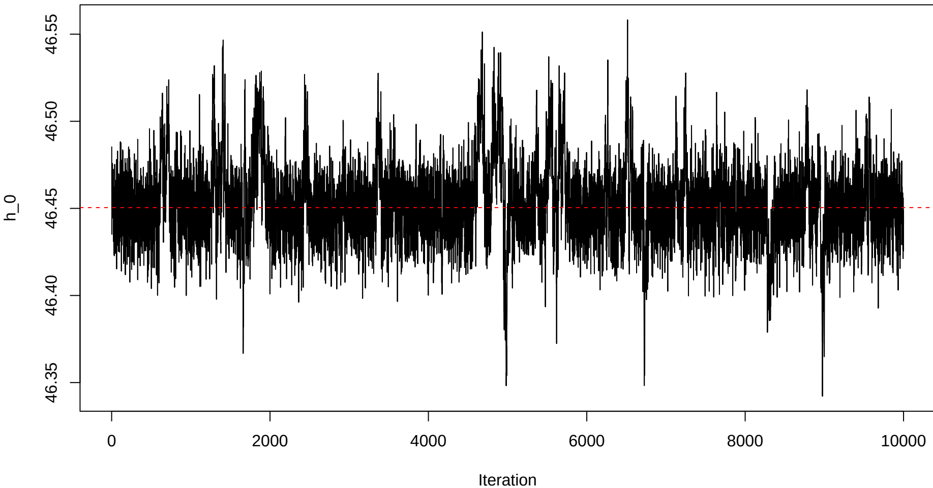
Trace plot – h0 – Sample 47
