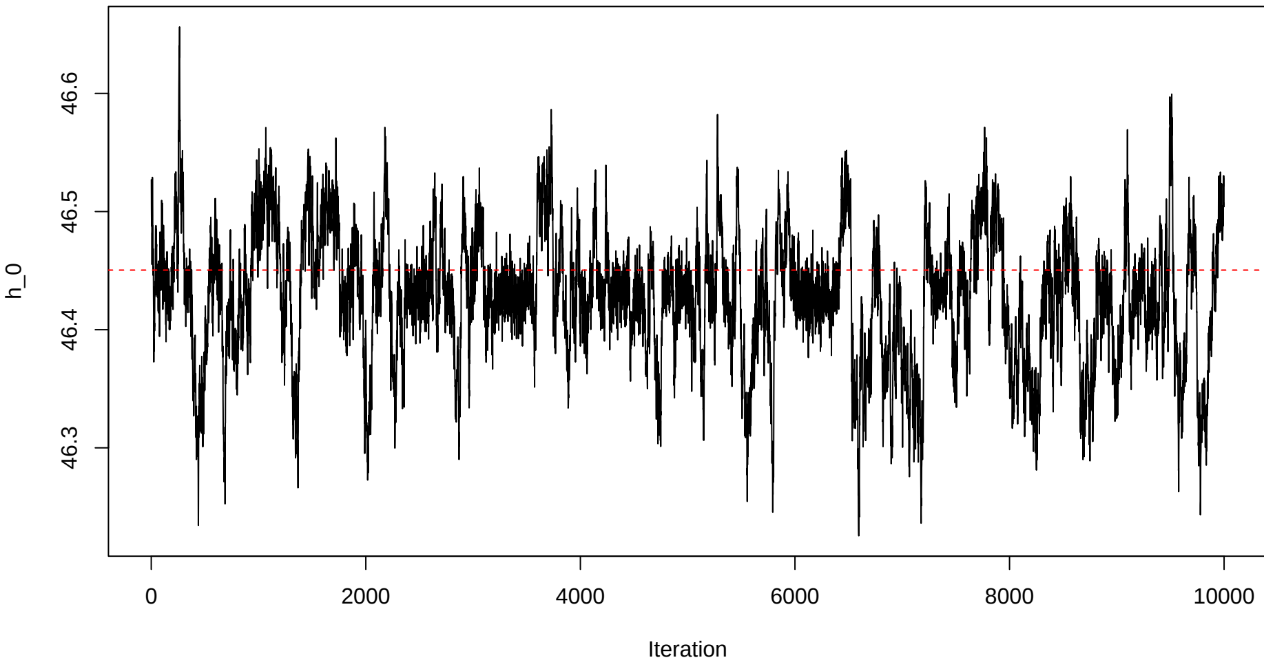
Trace plot – h0 – Sample 21
