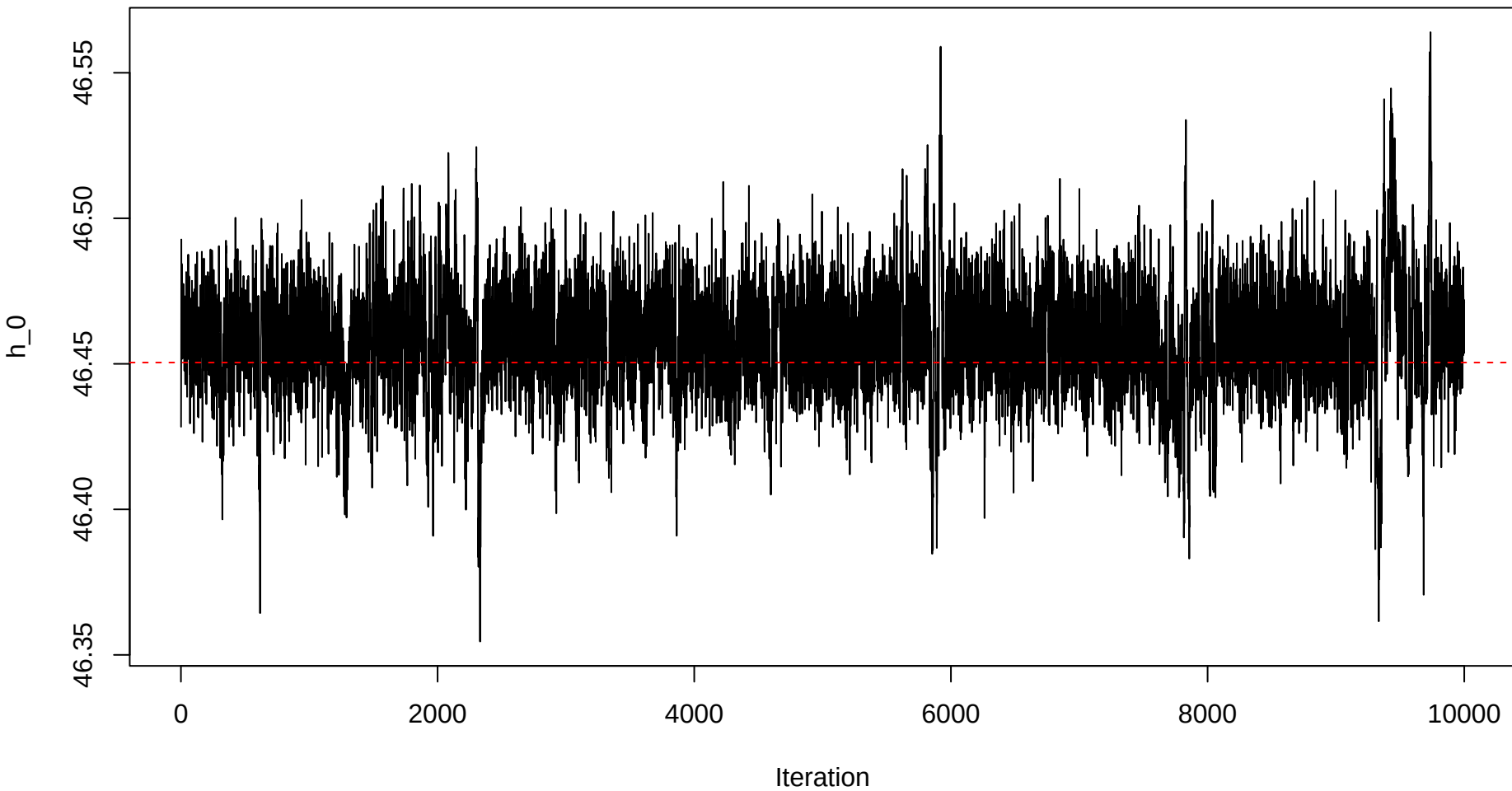
Trace plot – h0 – Sample 49
