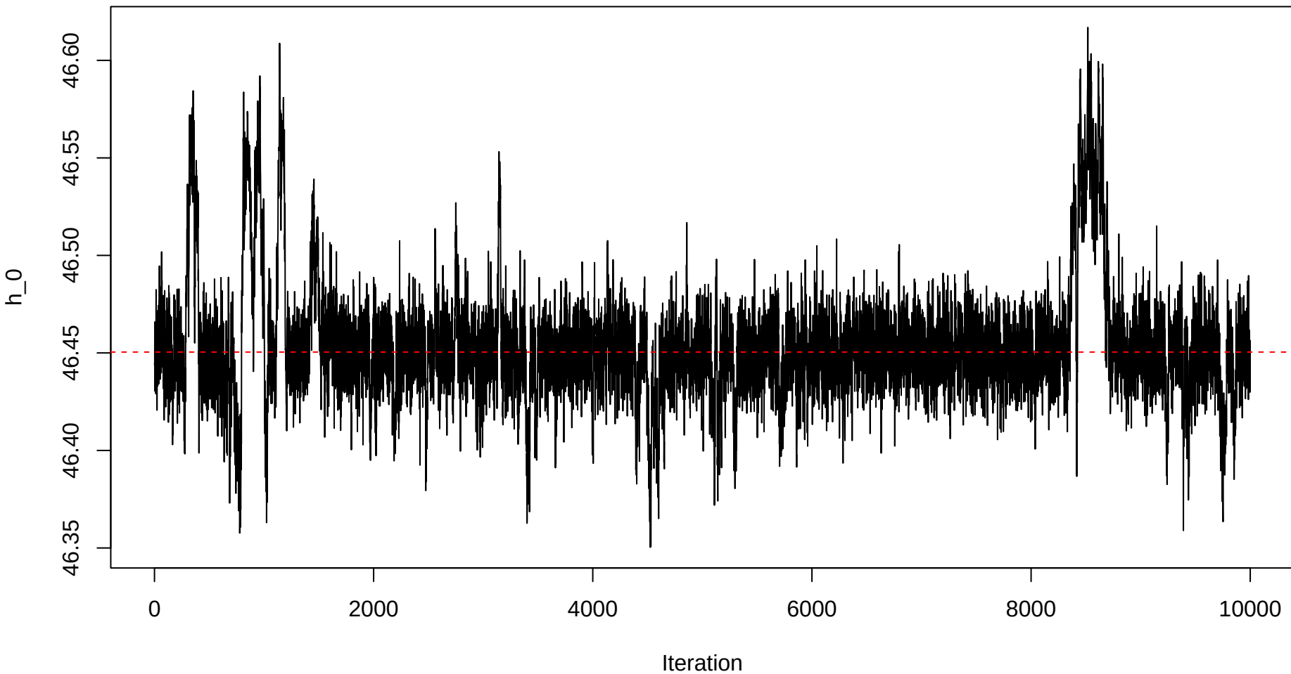
Trace plot – h0 – Sample 20
