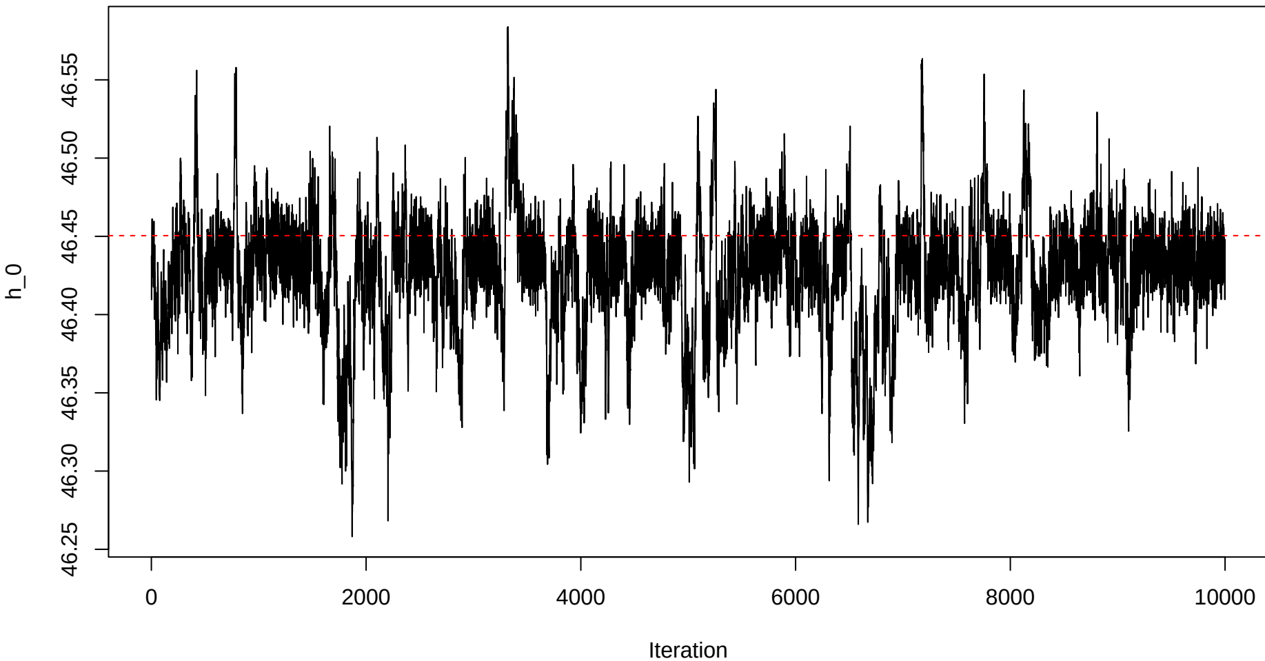
Trace plot – h0 – Sample 19
