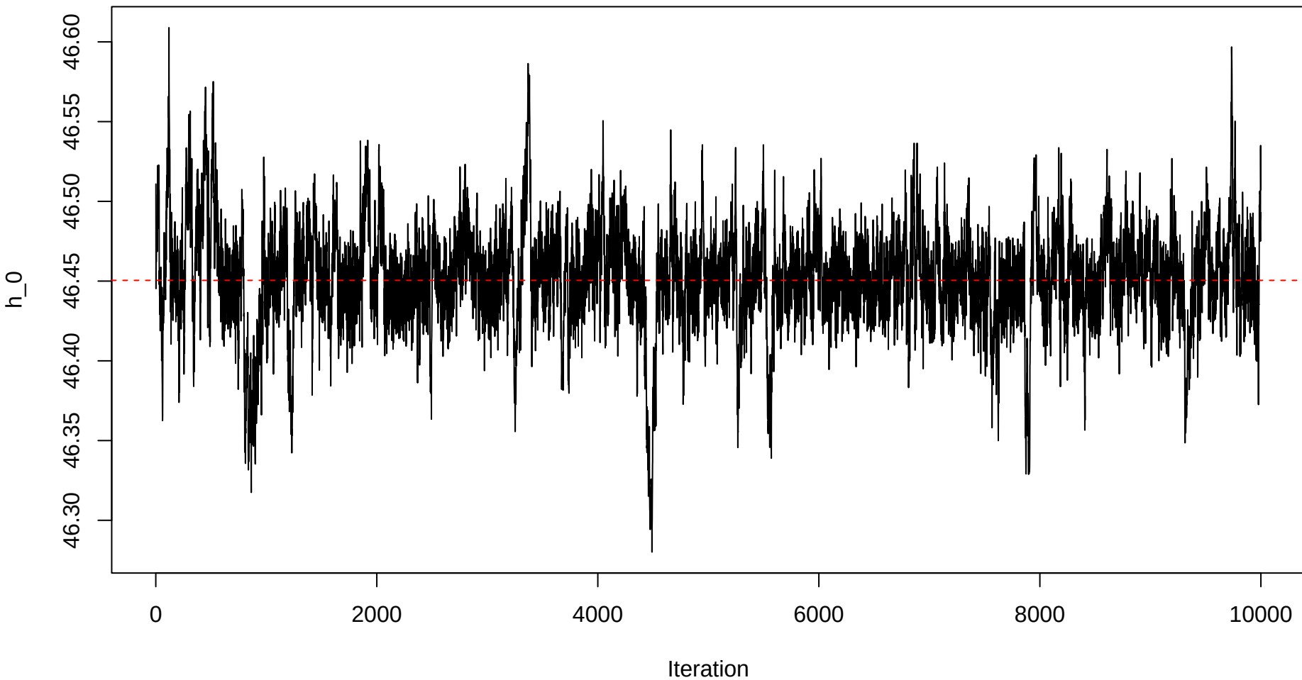
Trace plot – h0 – Sample 43
