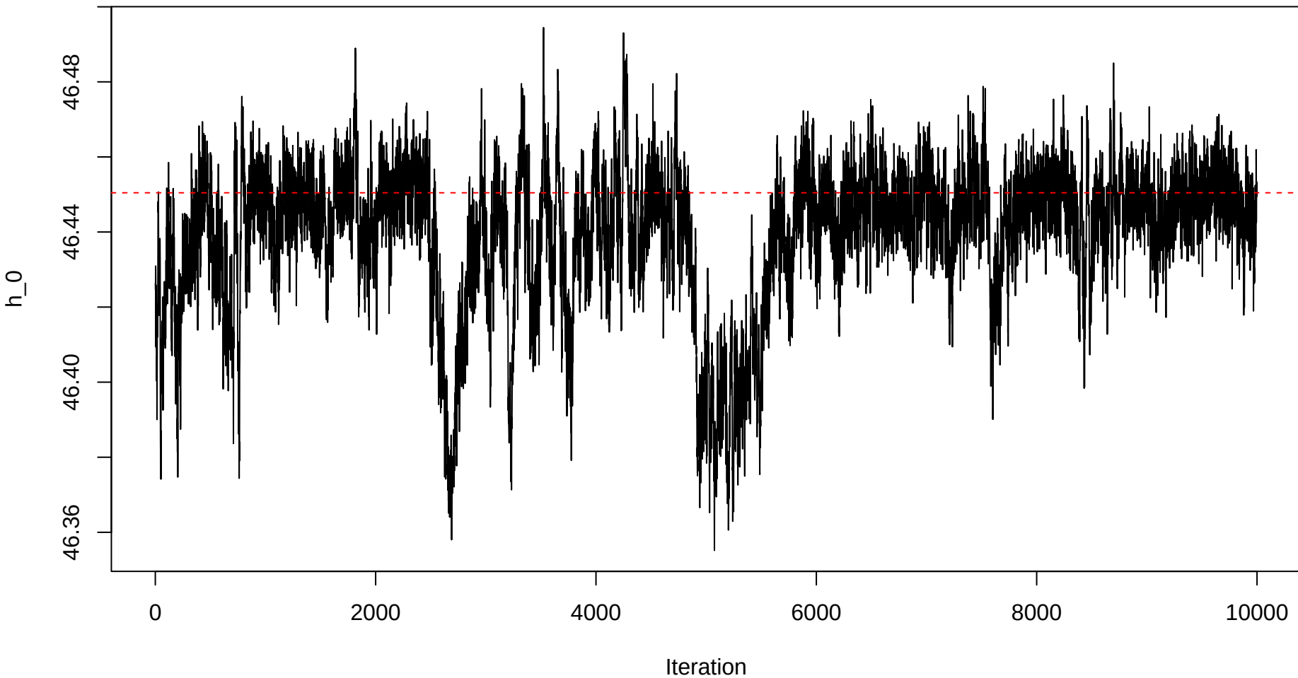
Trace plot – h0 – Sample 37
