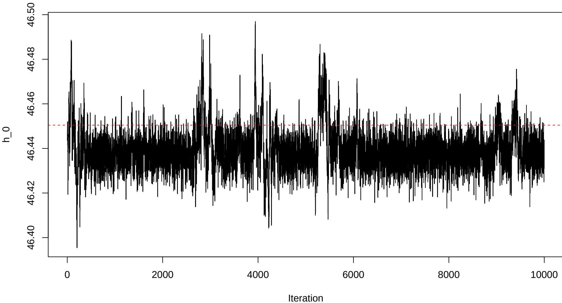
Trace plot – h0 – Sample 43
