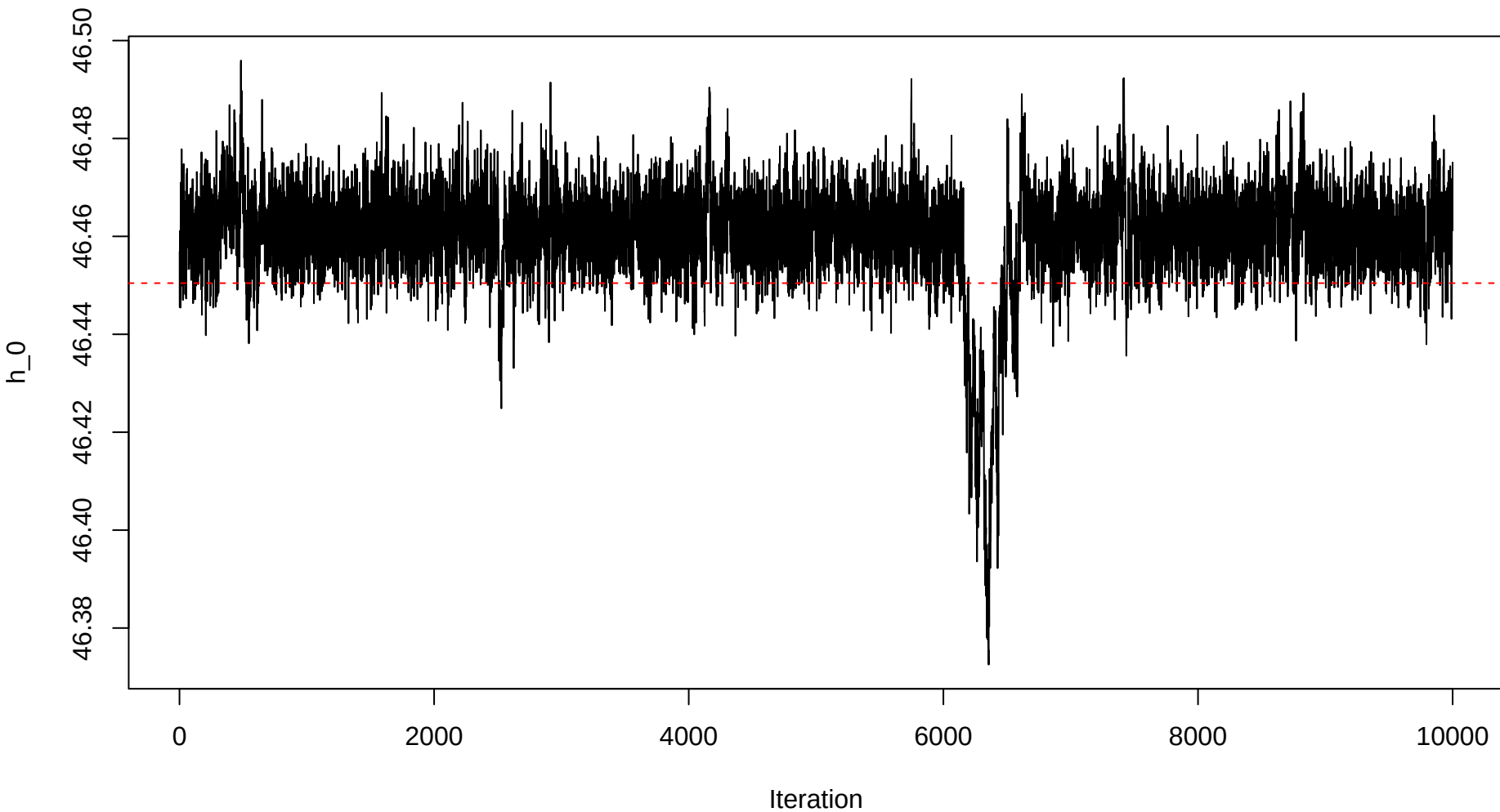
Trace plot – h0 – Sample 46
