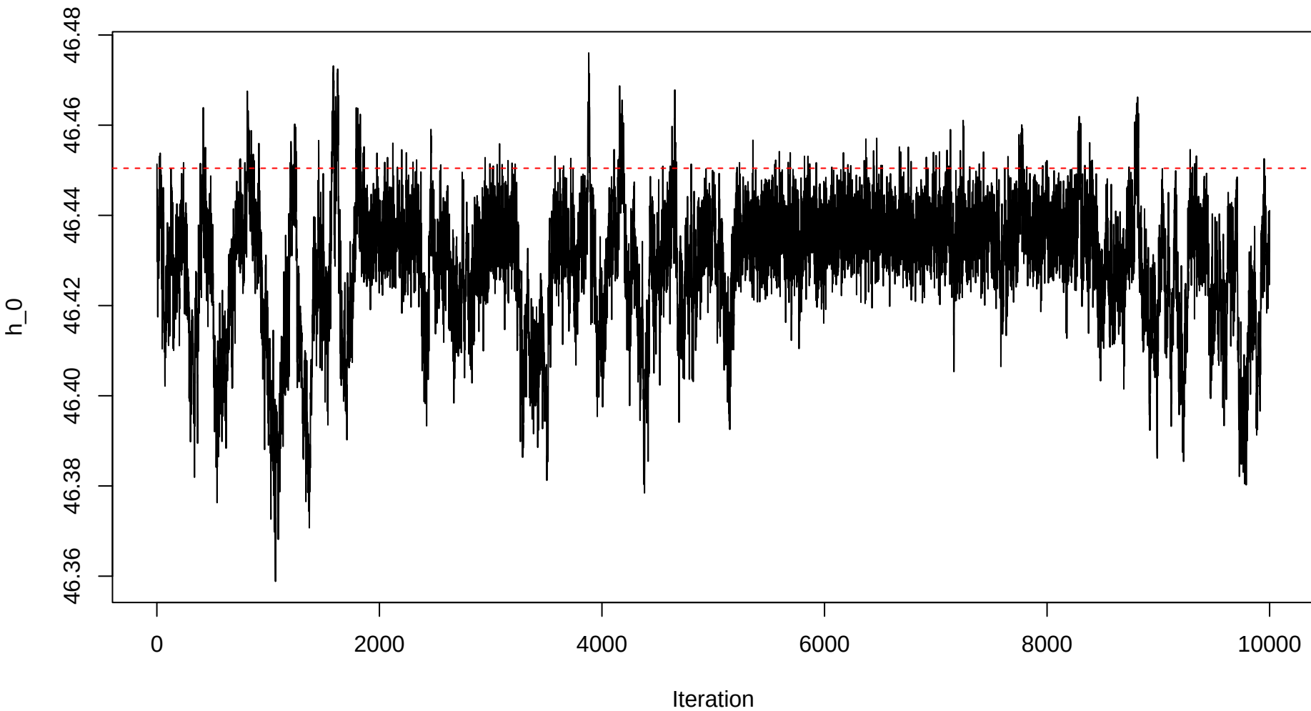
Trace plot – h0 – Sample 11
