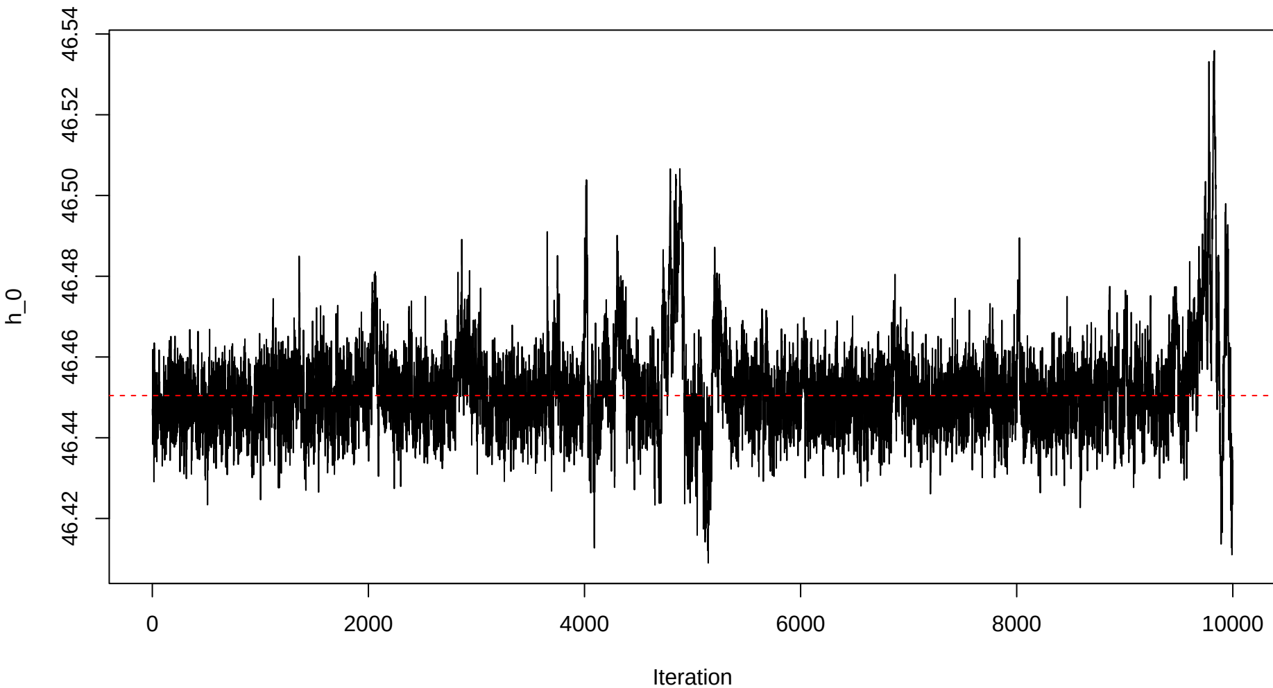
Trace plot – h0 – Sample 33
