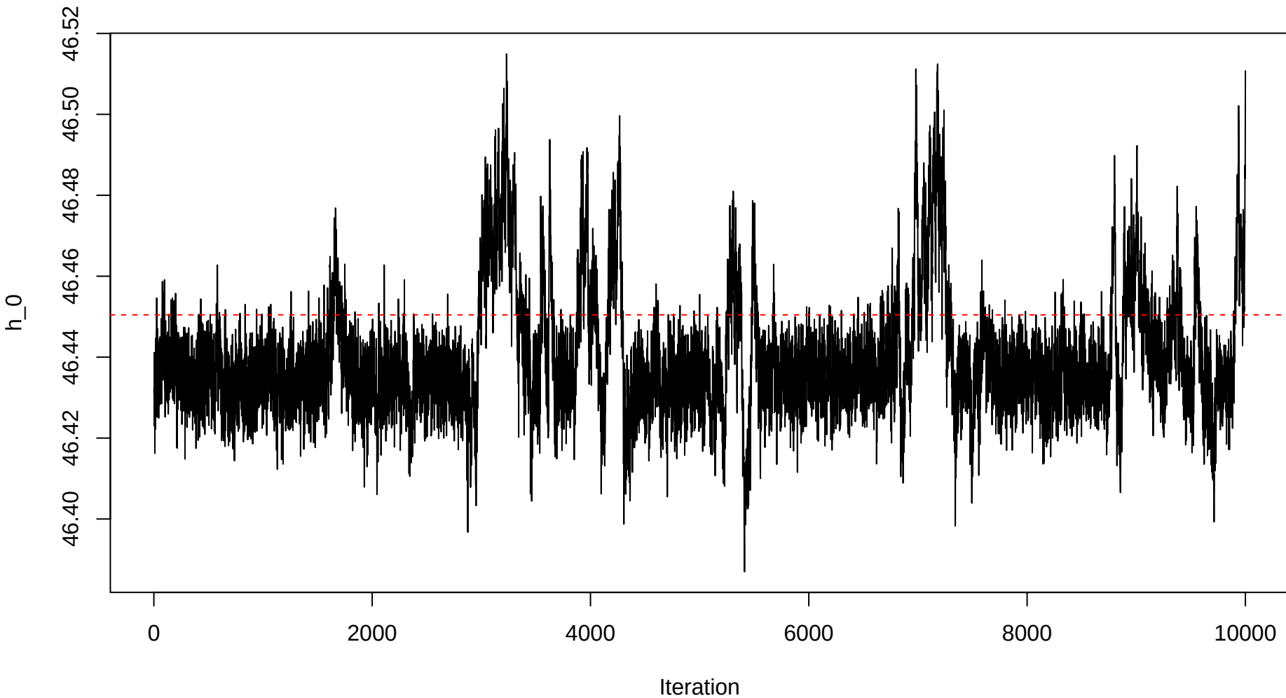
Trace plot – h0 – Sample 47
