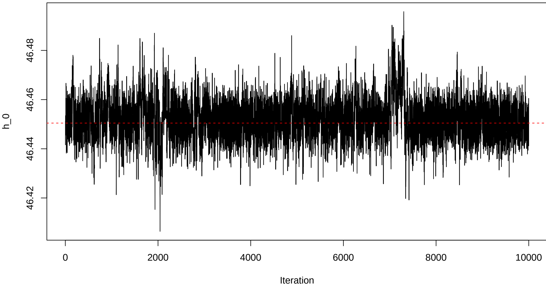
Trace plot – h0 – Sample 30
