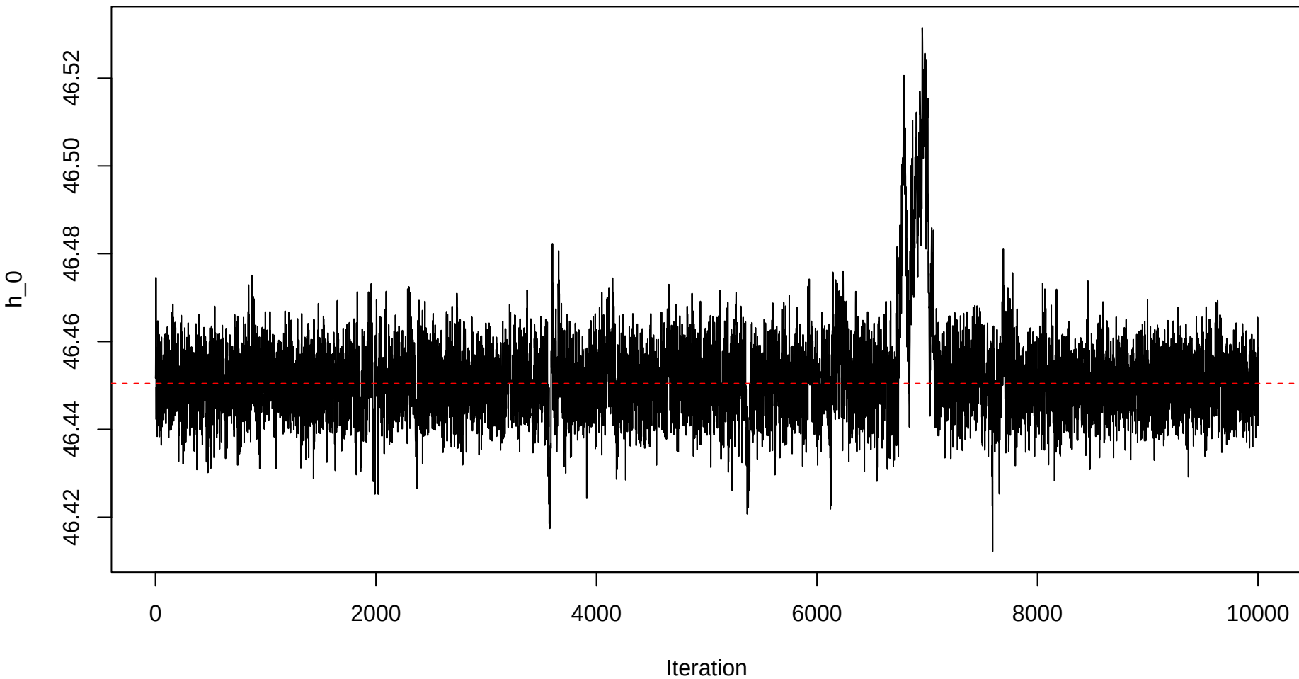
Trace plot – h0 – Sample 14
