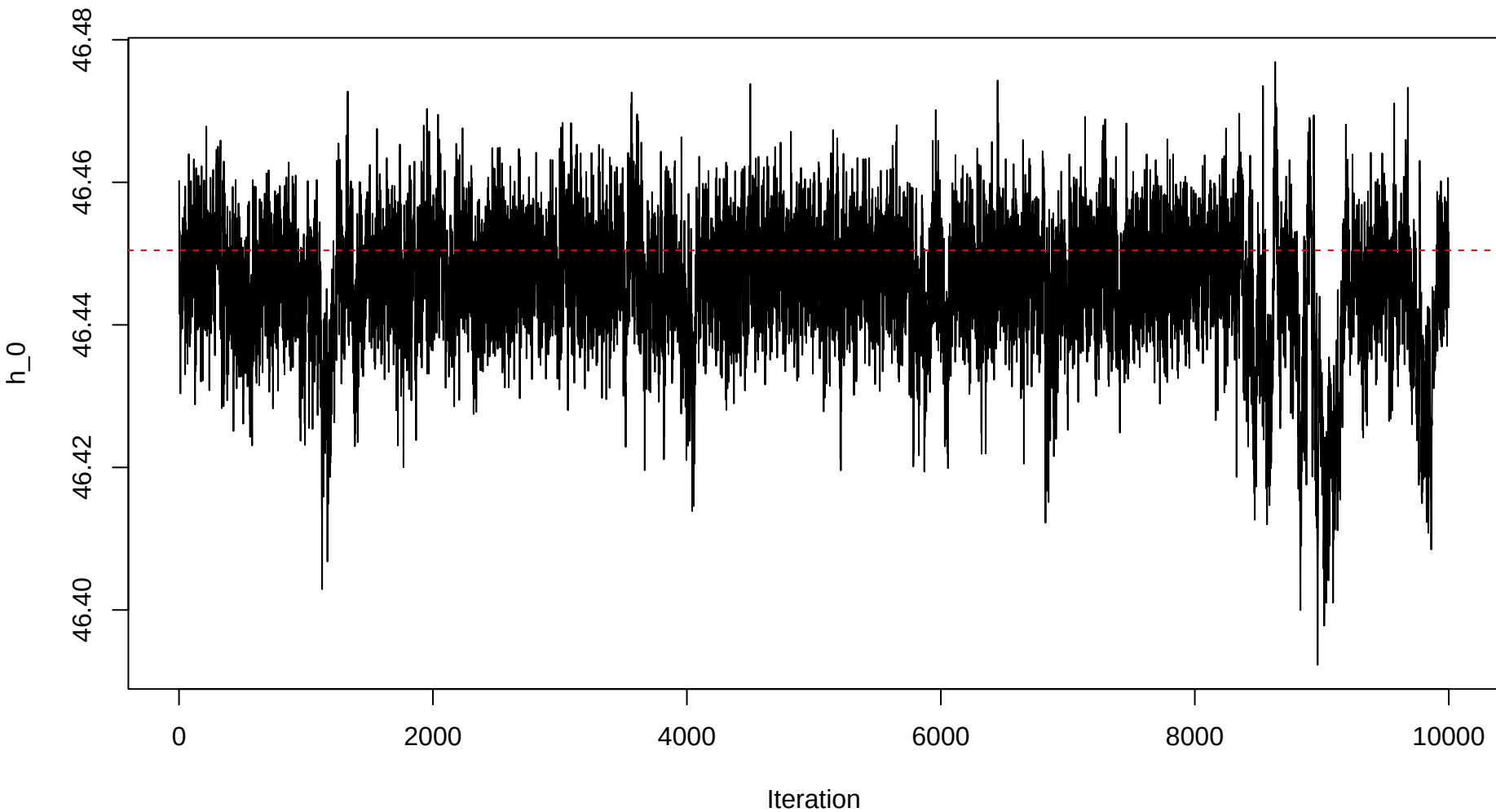
Trace plot – h0 – Sample 20
