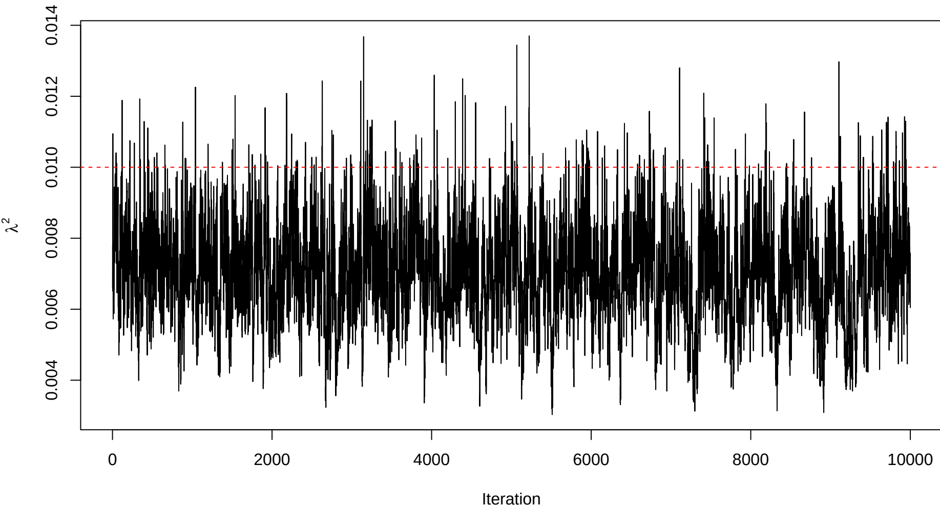
Trace plot – sigma_sq_err – Sample 13
