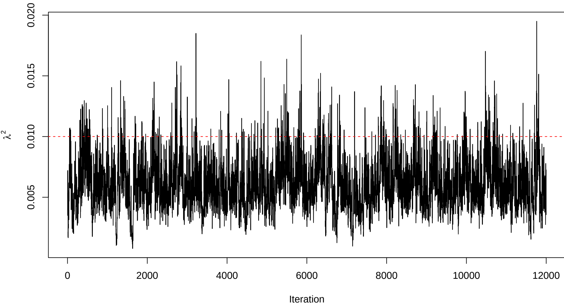
Trace plot – sigma_sq_err – Sample 49
