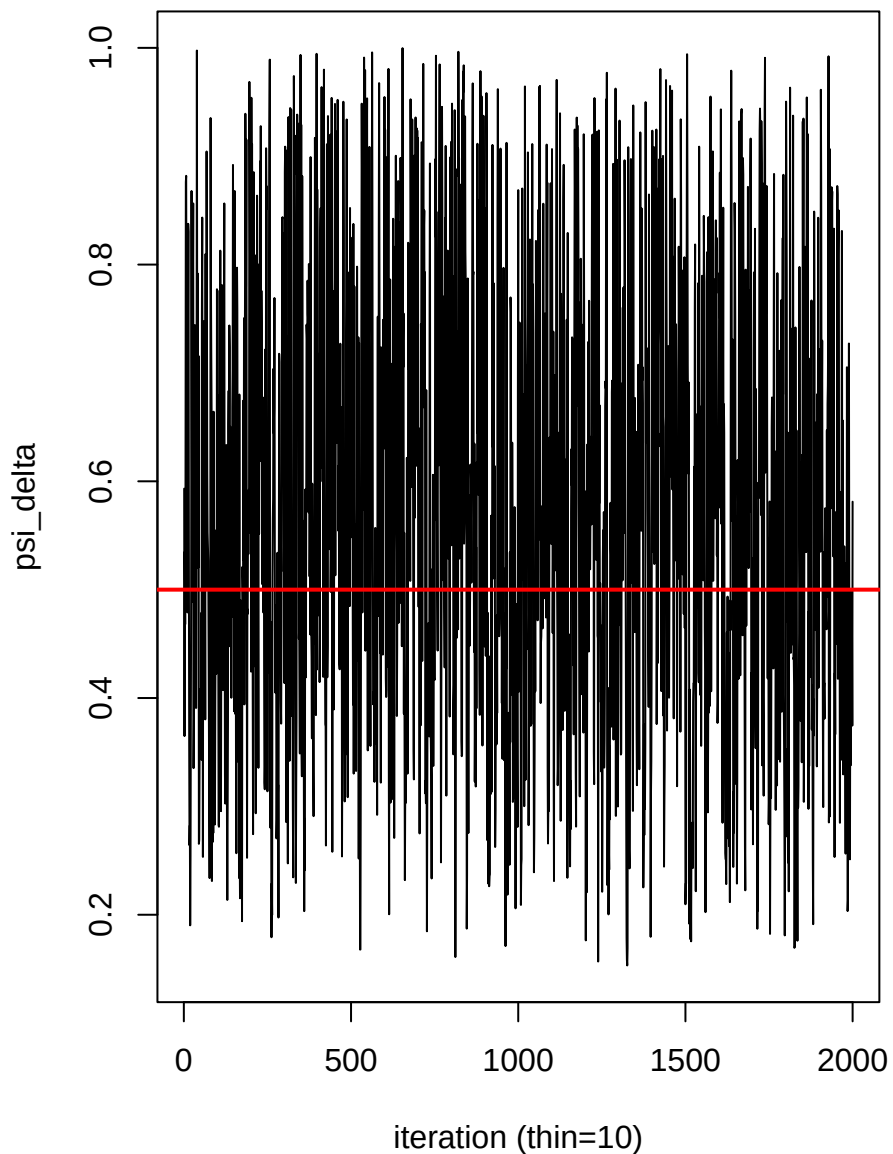
Trace plot: \psi_{\text{delta}}
