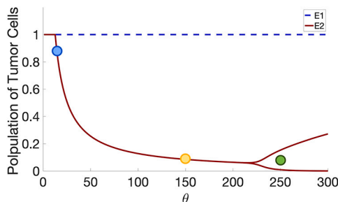
Fig. 1. Bifurcation diagram of the model (4) with bifurcation parameter \theta . The equilibrium E_1 loses stability at \theta \approx 12.7 , while E_2 becomes biologically relevant and remains stable up to the Hopf bifurcation at \theta_H \approx 220 . Beyond this point, the system exhibits oscillatory dynamics. The parameter values used here are a = 0.96 and \gamma = \frac{40}{3} . The circles mark the \theta values selected in Section 5 for numerical simulations.
