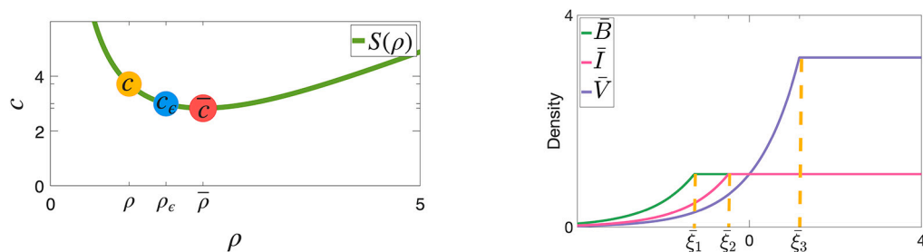
Fig. 3. Left: Wave-speed function S(\rho) together with the values \bar{c} , c , and c_\epsilon . The point (\bar{\rho}, \bar{c}) is marked in red. The points \rho = \bar{\rho} - \tau and \rho_\epsilon = \rho + \epsilon , with \tau = 1 and \epsilon = 0.5 , are also shown, along with their corresponding wave speeds (c, c_\epsilon) . Right: Sketch of the upper solutions and their transition points \bar{\xi}_1 , \bar{\xi}_2 , and \bar{\xi}_3 .
