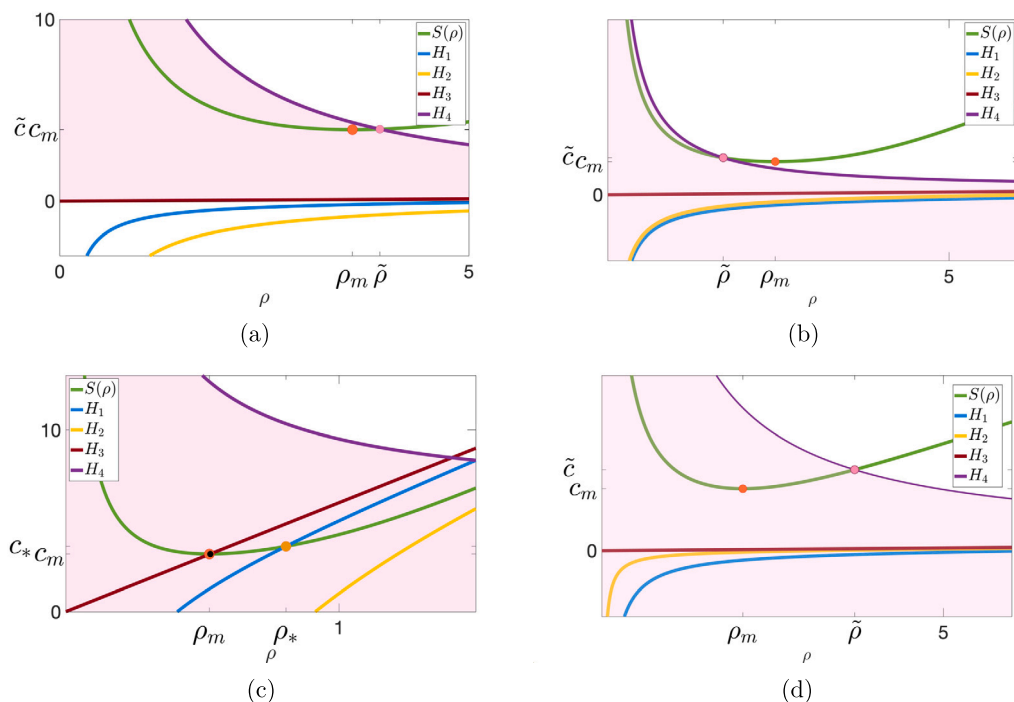
Fig. 2. Numerical illustration of S(\rho) , and its minimum value indicated by the orange ball, and H_1(\rho) , H_2(\rho) , H_3(\rho) , and H_4(\rho) for different parameter values. The parameter values have been chosen to illustrate each of the regimes and are given by: (a) a = \frac{10}{3} , \gamma = \frac{40}{3} , \theta = 250 , D = 0.025 (b) a = 0.96 , \gamma = \frac{40}{3} , \theta = 50 , D = 0.025 , (c) a = 5 , \gamma = 2 , \theta = 17 , D = 6 (d) a = 0.96 , \gamma = 1.25 , \theta = 17 , D = 0.025 . Note that case (c) may not arise in biologically relevant cases. (For interpretation of the colours in the figure(s), the reader is referred to the web version of this article.)
