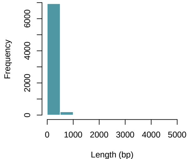
DMR length distribution
