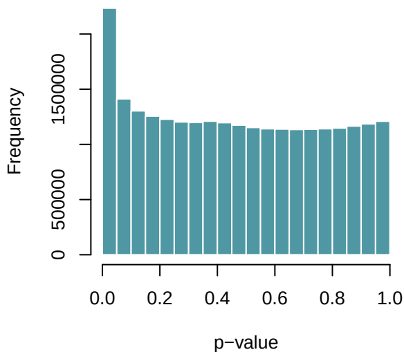
MID_vs_YOUNG – p-value distribution
