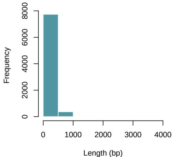
DMR length distribution
