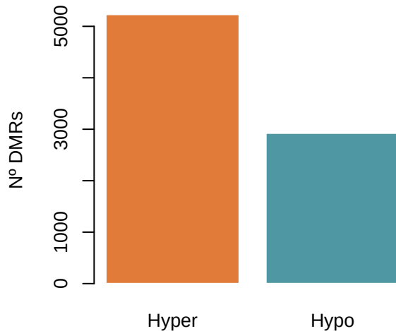
DMRs: OLD_vs_MID
