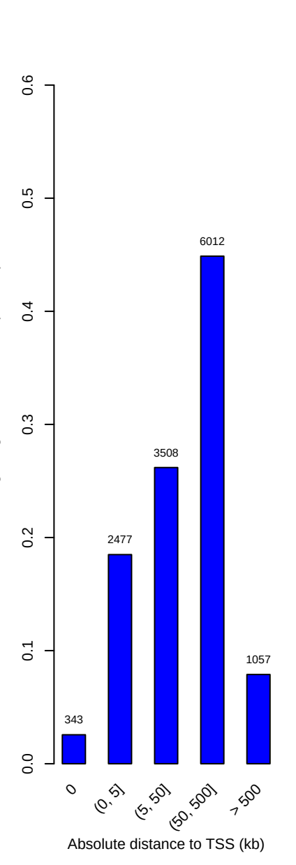
Binned by absolute distance to TSS
