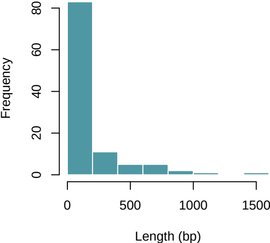
DMRs: OLD_vs_YOUNG
