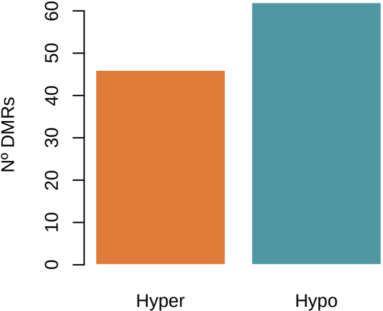
DMRs: OLD_vs_YOUNG
