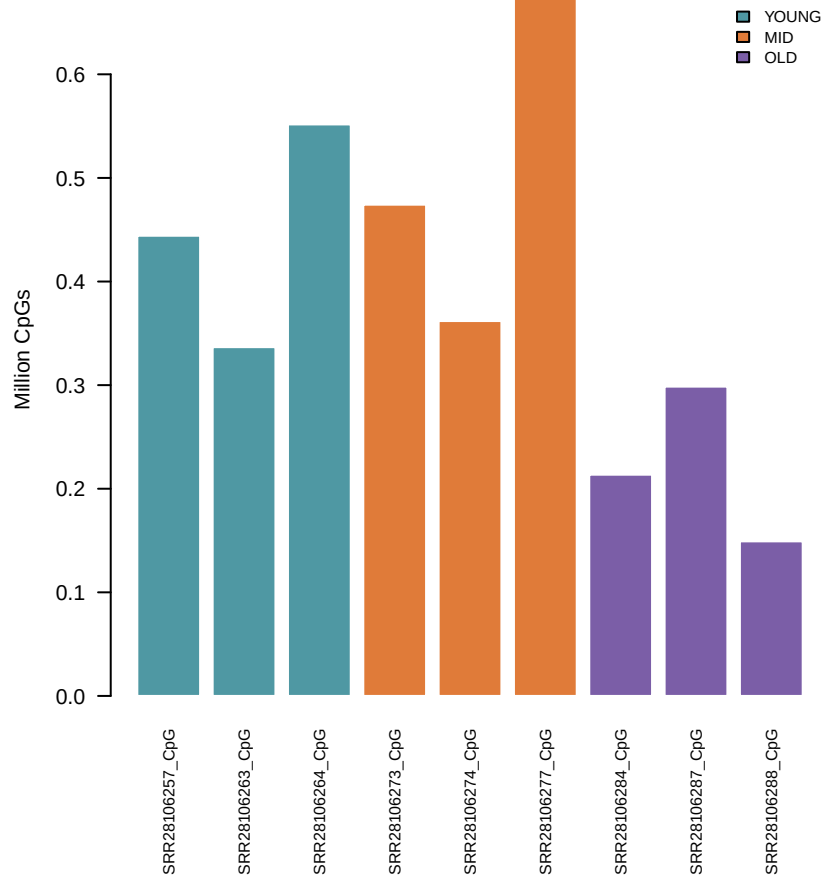
CpG cumulative coverage
