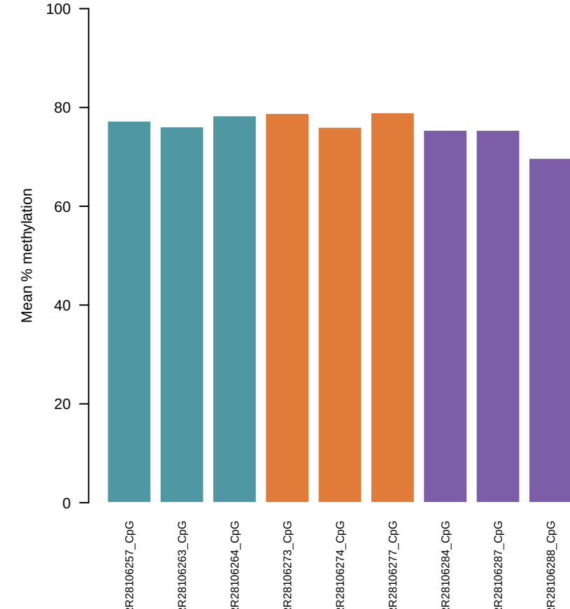
Global CpG methylation per sample
