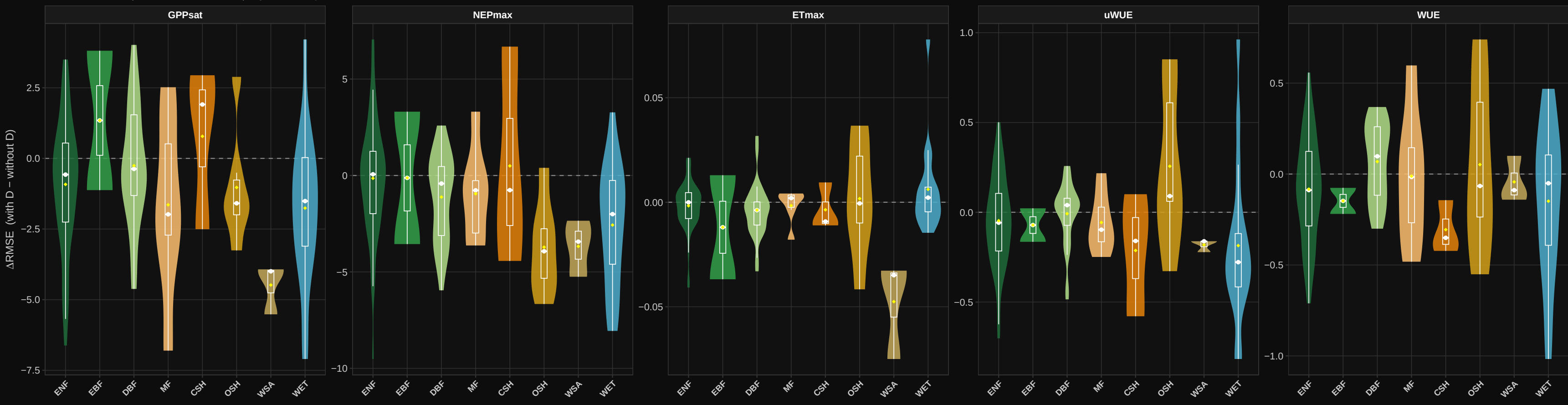
Effect of adding disturbance on per-site RMSE by IGBP class ... M5vsM6_anom_24m
