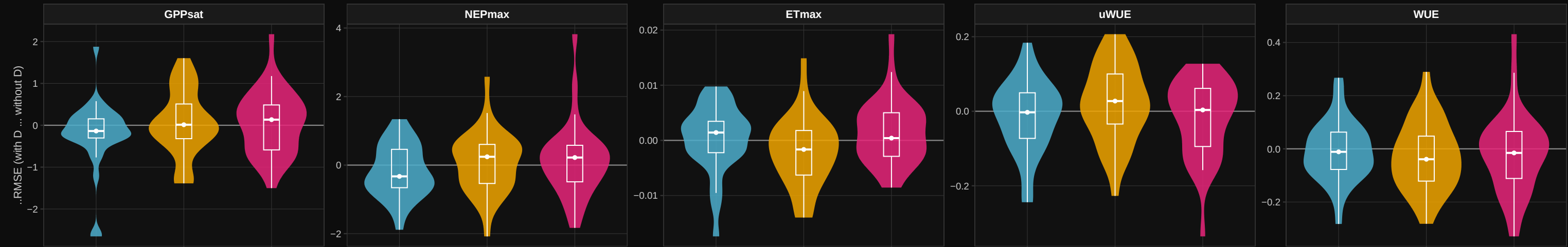
Relative Disturbance
