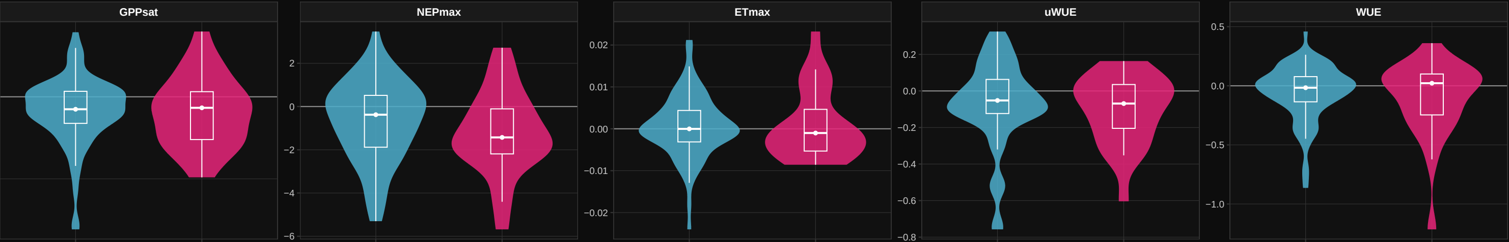
Relative Disturbance
