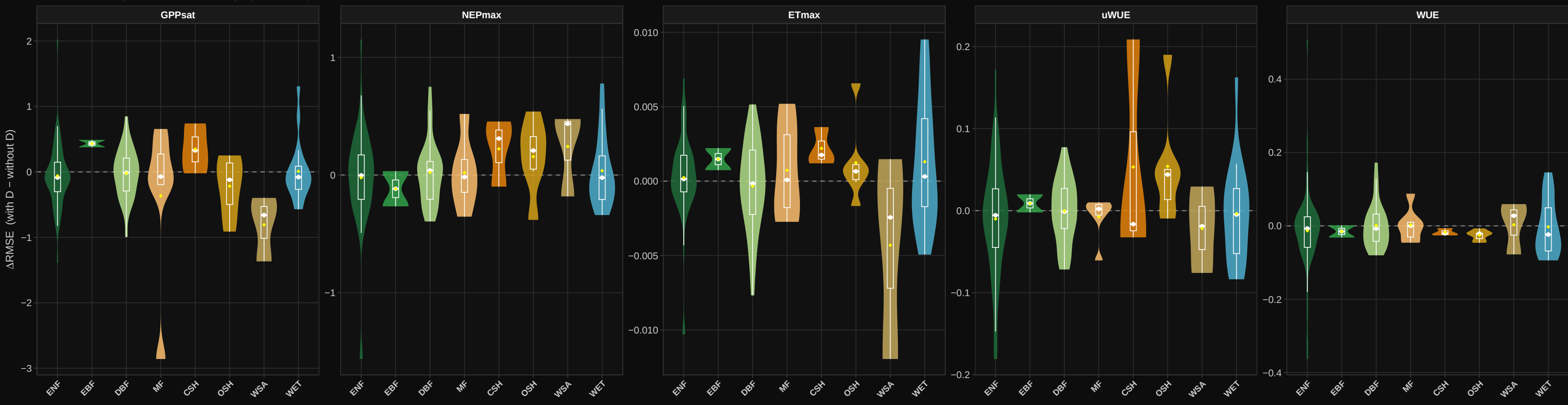
Effect of adding disturbance on per-site RMSE by IGBP class ... M7vsM8_raw_12m
