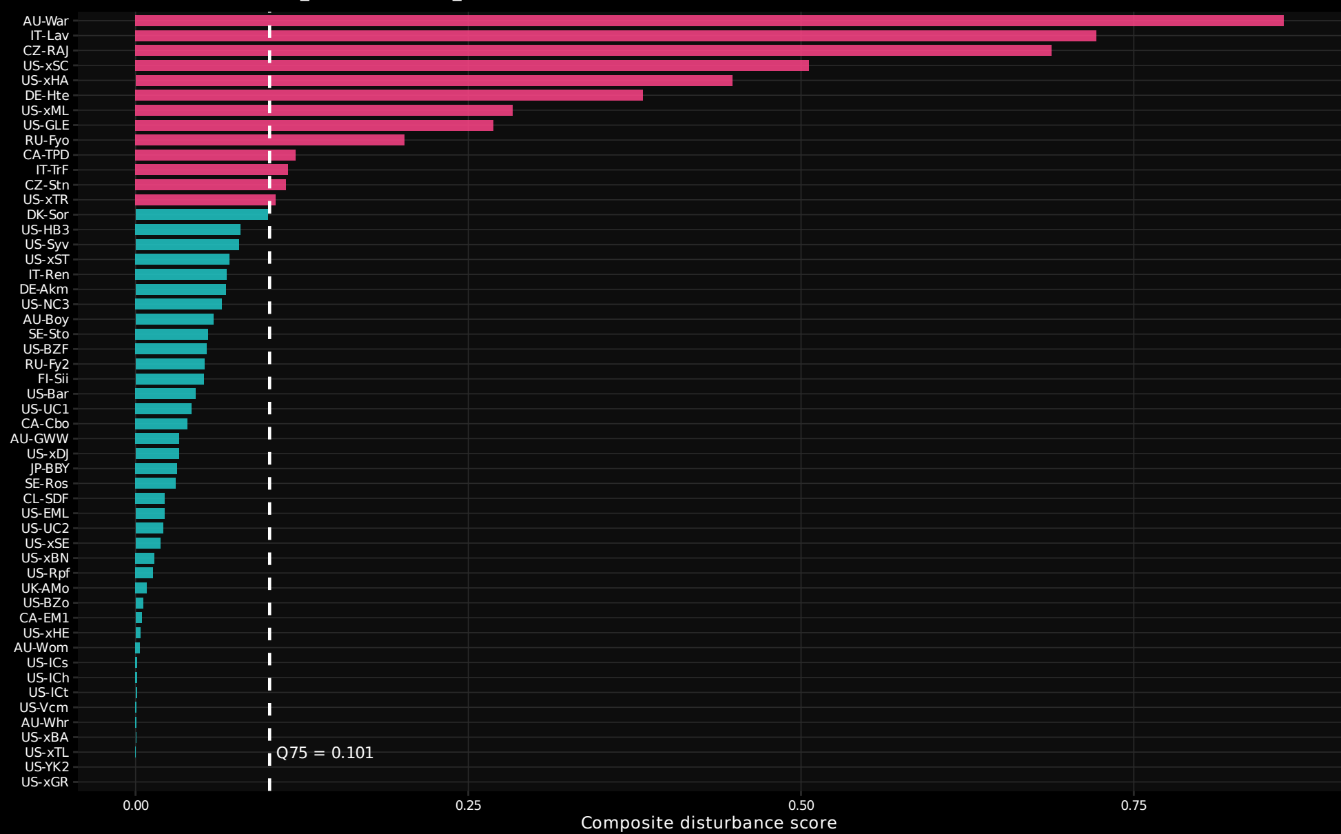
C Site ranking by composite score (0.5 × loss + 0.4 × dw_inc + 0.1 × dw_mean)
