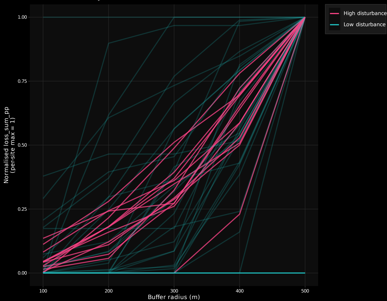
D Buffer sensitivity of forest loss
