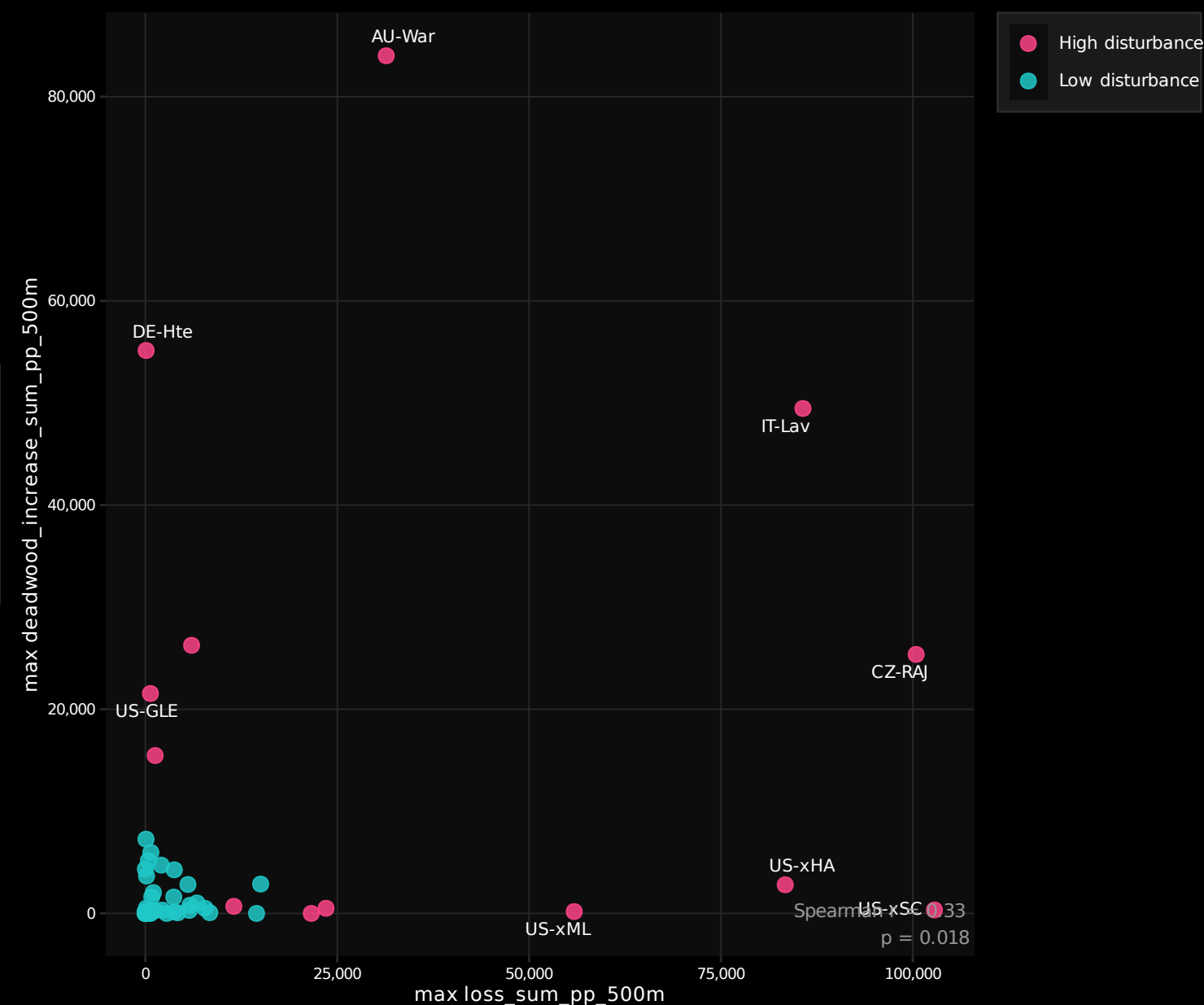
D Buffer sensitivity of forest loss
