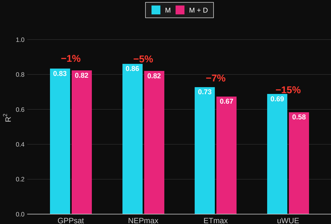
R^2 comparison: M vs M + D [24m window, raw-lag memory]
