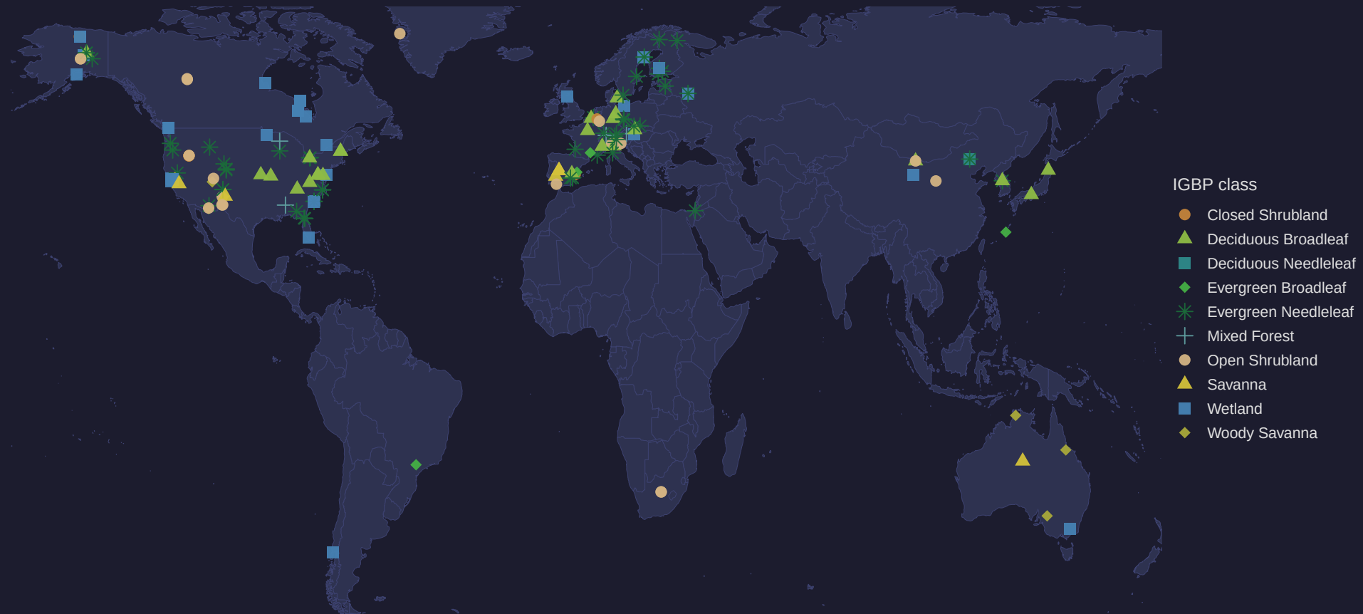
Study sites (n = 166) – IGBP land-cover class
