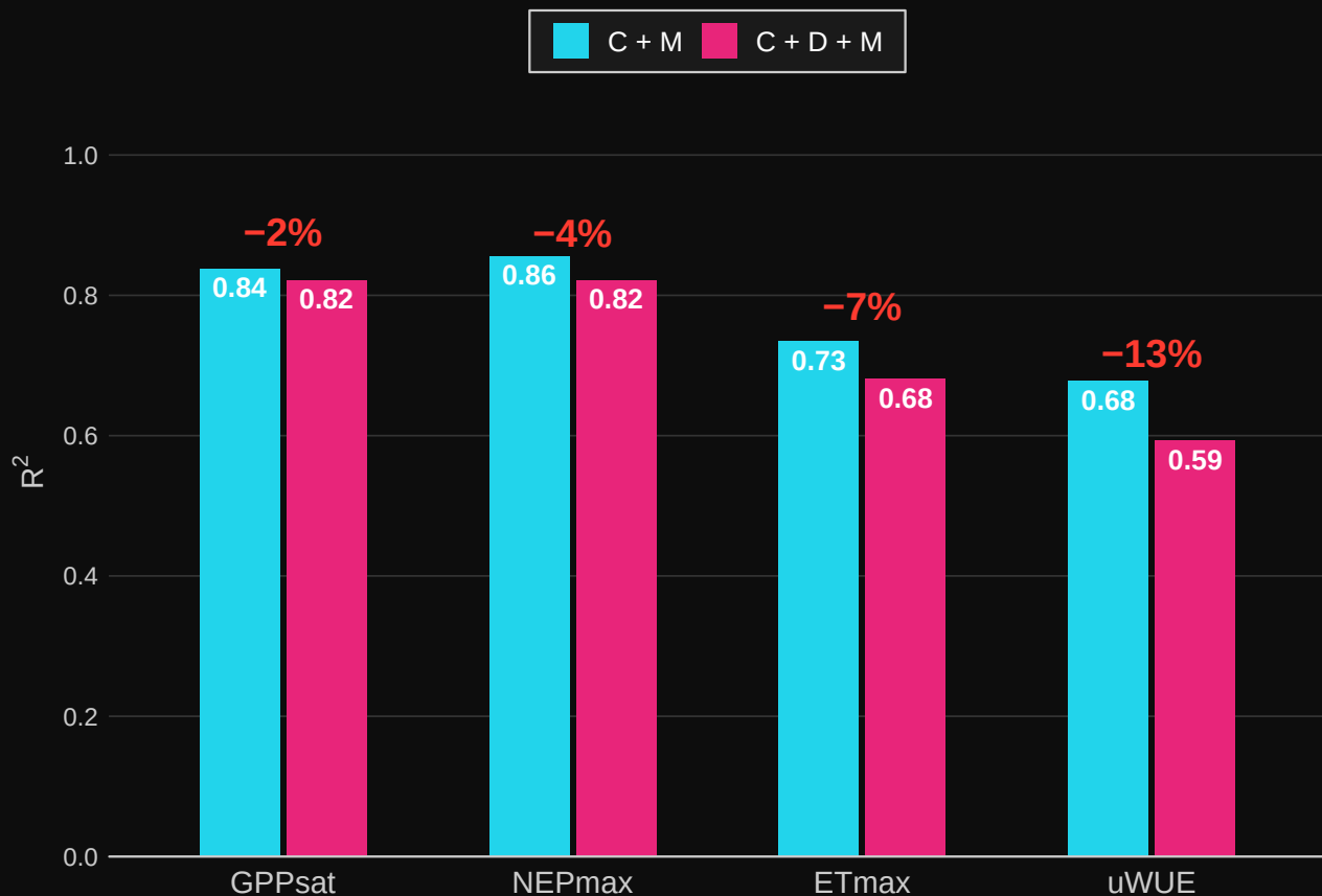
R 2 comparison: C + M vs C + D + M [24m window, raw-lag memory]
