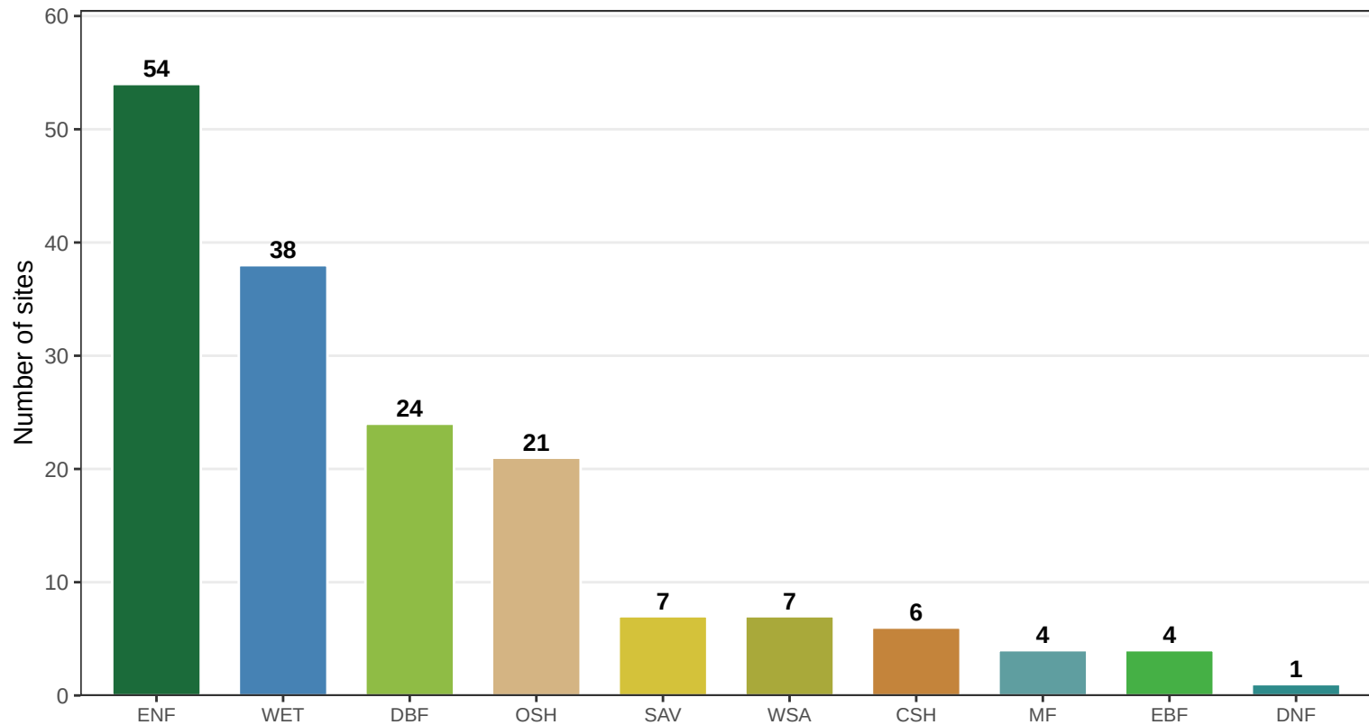
Sites per IGBP class (n = 166 total)
