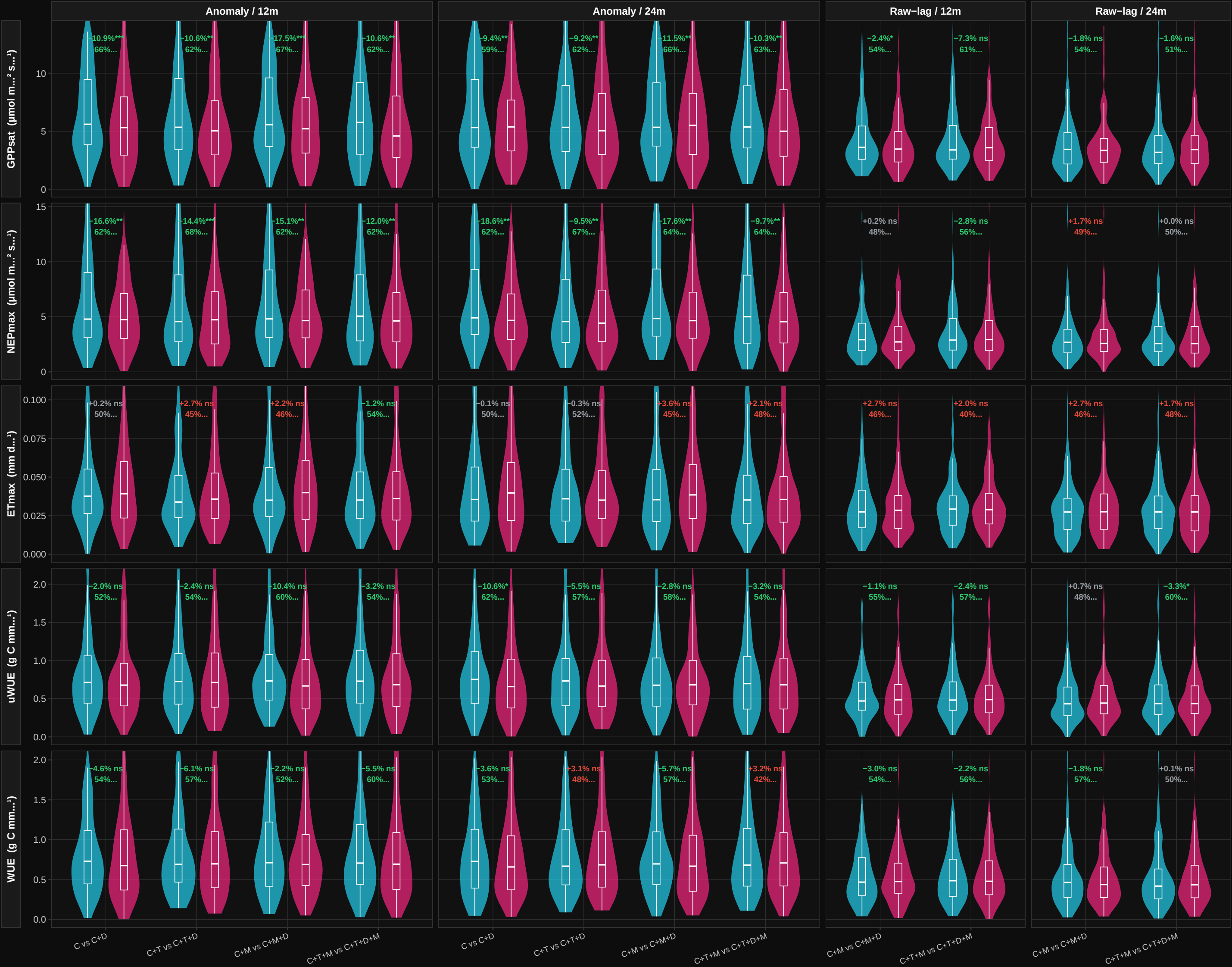
Effect of adding deadwood disturbance on per-site RMSE Paired violin: cyan = without D, pink = with D | LO SO CV | 112 sites | % = MEDIAN PAIRED change in per-site RMSE (negative = less error, green) stars = one-sided paired Wilcoxon, H1: adding D reduces RMSE, BH-FDR within figure (** q<0.001, ** q<0.01, * q<0.05, ns) y axis zoomed to the 95th percentile – no data removed; M1–M4 have no memory term and appear once, under Anomaly
