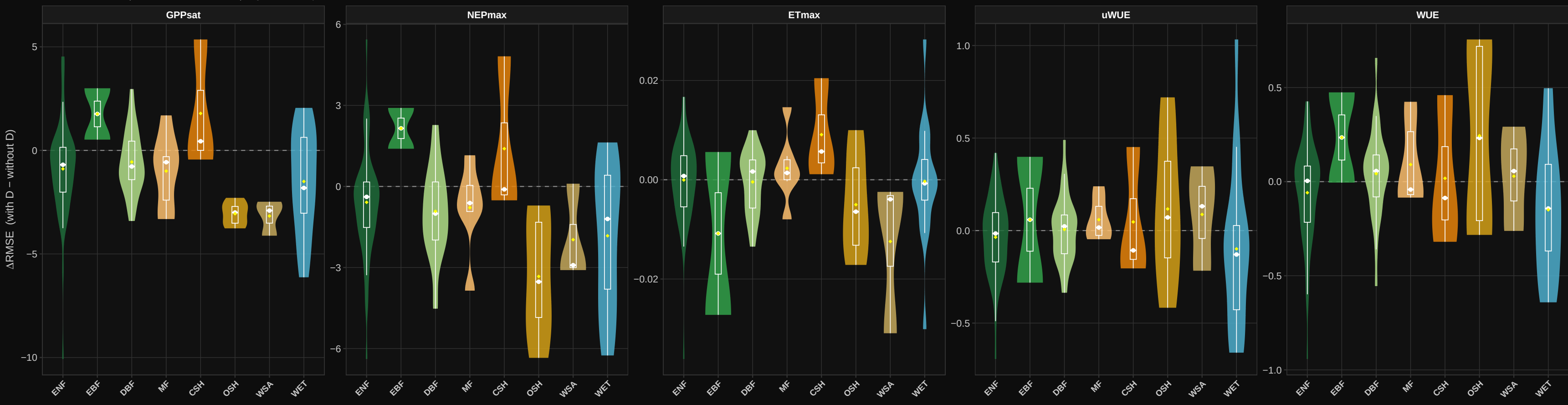
Effect of adding disturbance on per-site RMSE by IGBP class ... M3vsM4_12m
