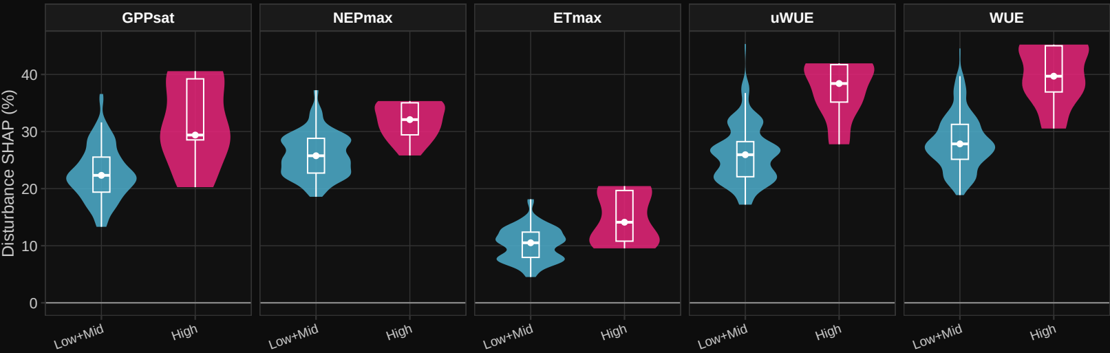
Disturbance SHAP % by Relative Mortality (M8_anom 12m)
