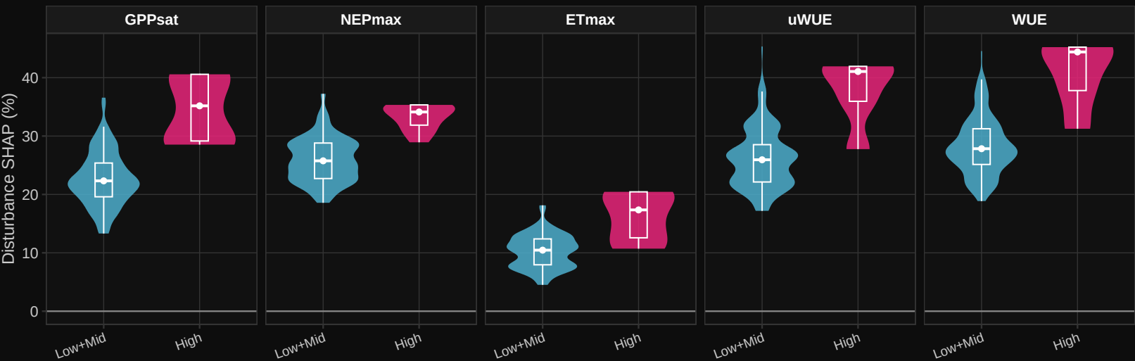
Disturbance SHAP % by Relative Disturbance (M8_anom 12m)
