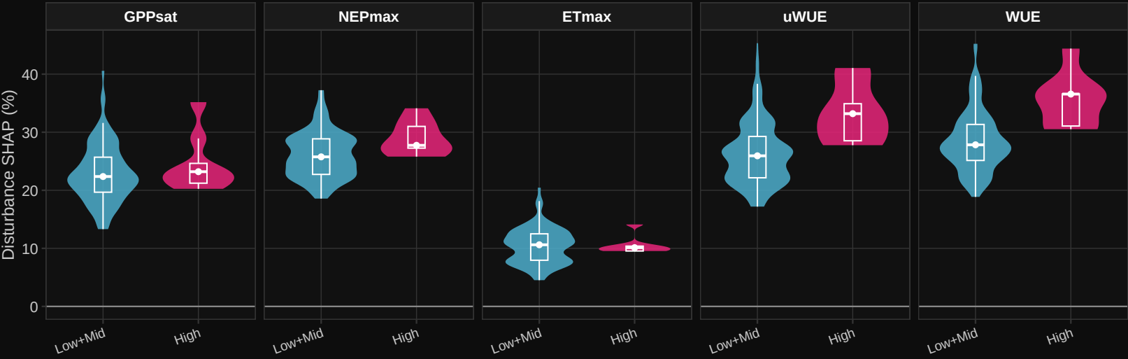
Disturbance SHAP % by Absolute Mortality (M8_anom 12m)
