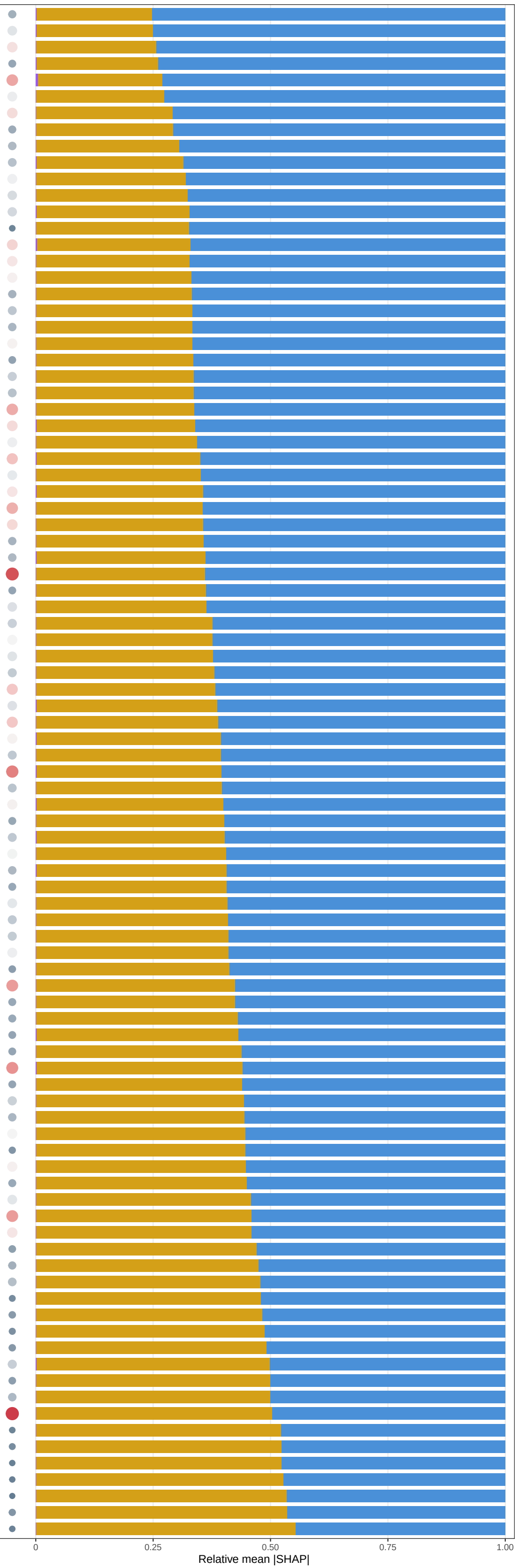
M6 anom (C+T+D+Mem) | 24m window | GPPsat ( \mu\text{mol m}^{-2} \text{s}^{-1} )
