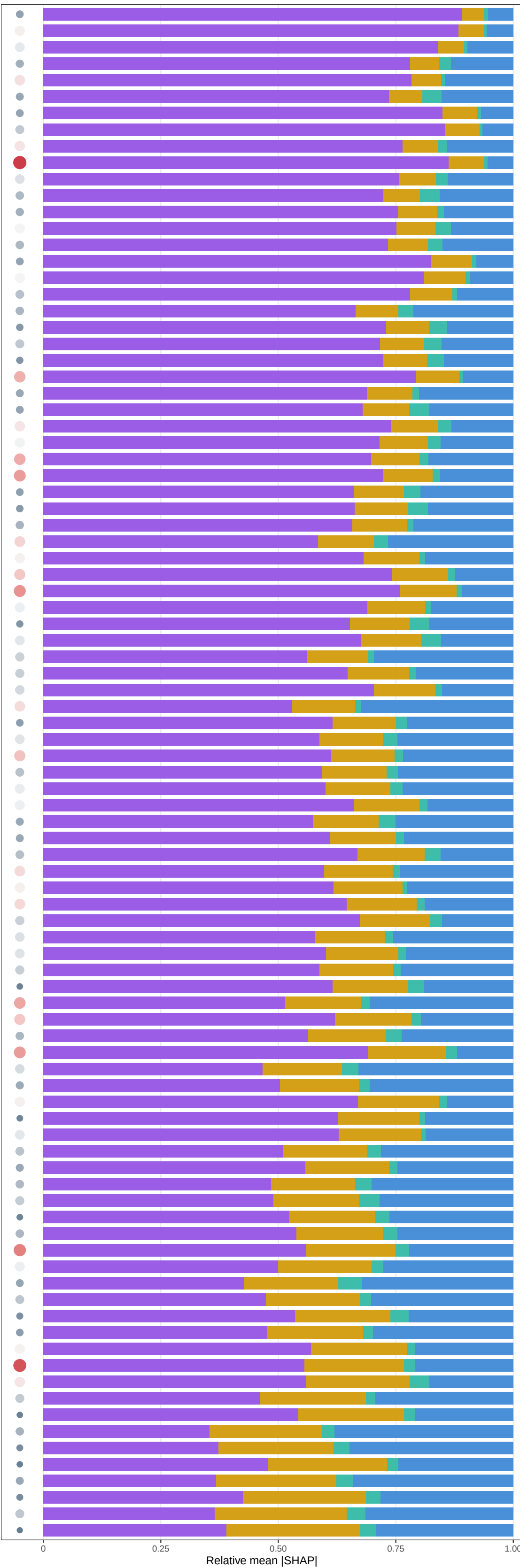
M8 raw (C+T+D+Mem) | 12m window | WUE (g C mm -1 )
