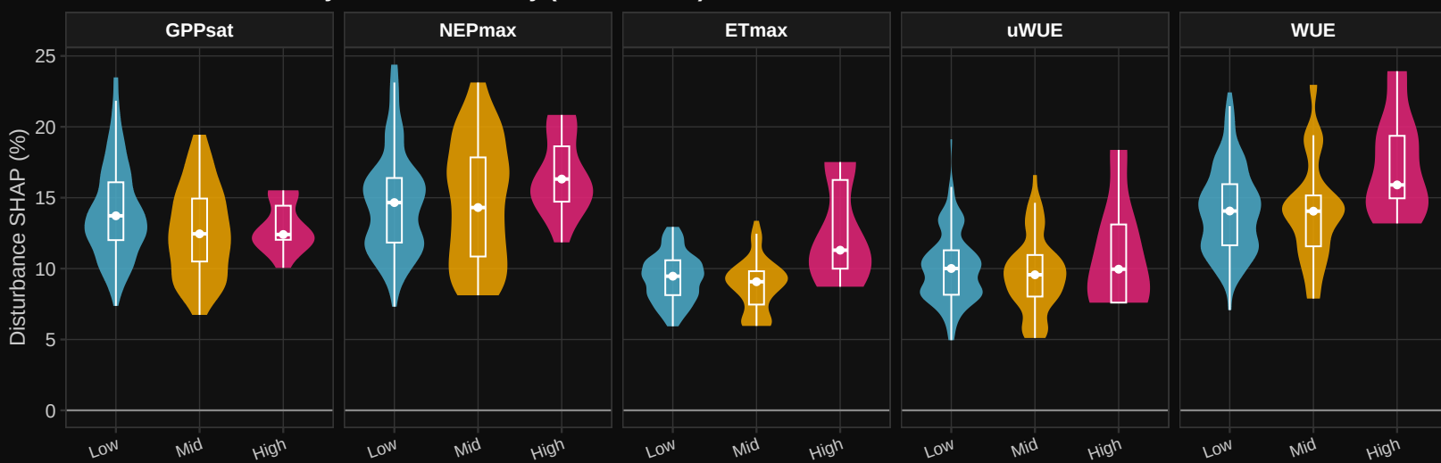
Disturbance SHAP % by Relative Mortality (M6_raw 24m)
