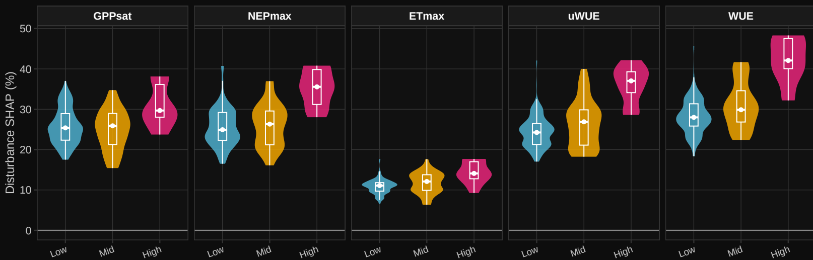
Disturbance SHAP % by Relative Mortality (M8_anom 12m)
