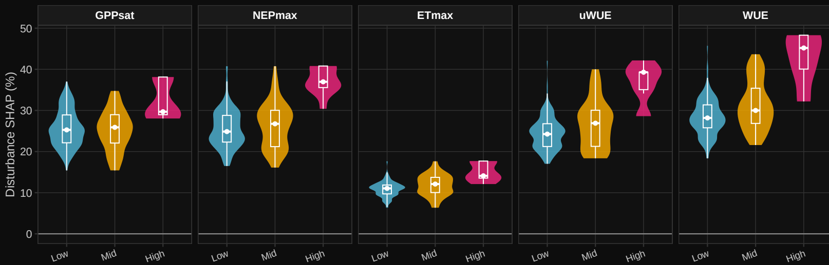
Disturbance SHAP % by Relative Disturbance (M8_anom 12m)
