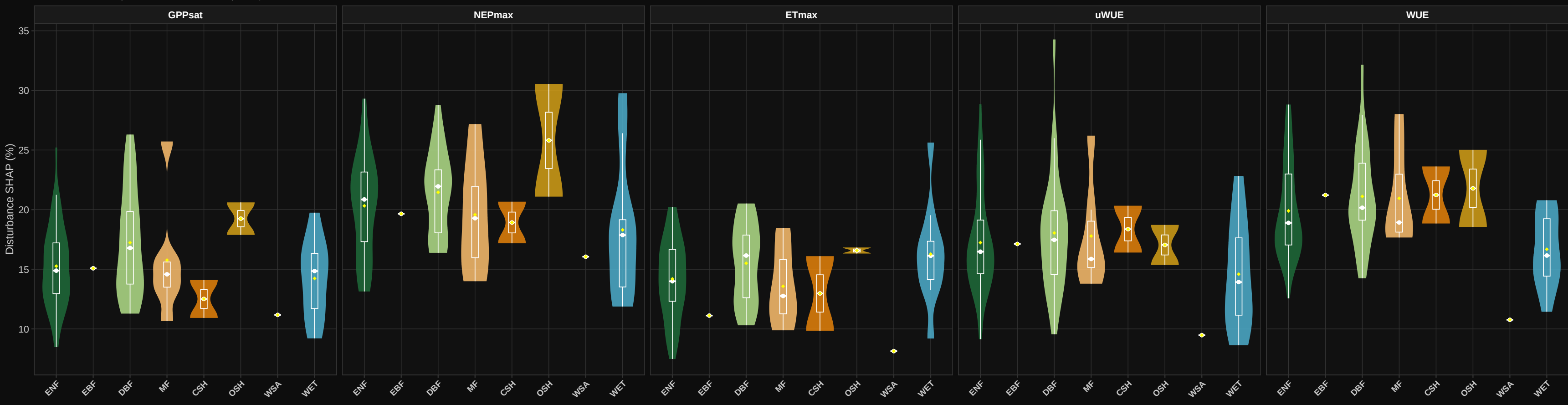
Disturbance SHAP % by IGBP class ... M6 raw (C+D+Mem) | 12m
