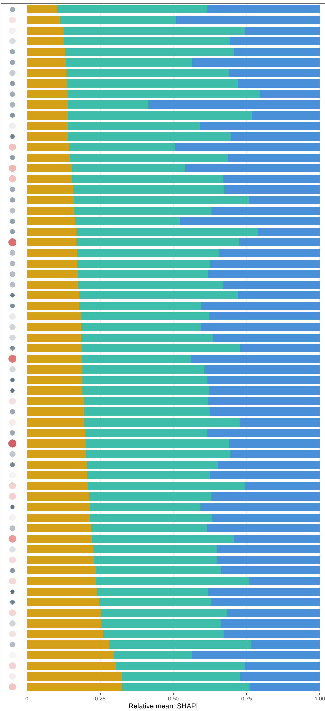
M4 (C+T+D) | 12m window | GPPsat ( \mu\text{mol m}^{-2} \text{s}^{-1} )
