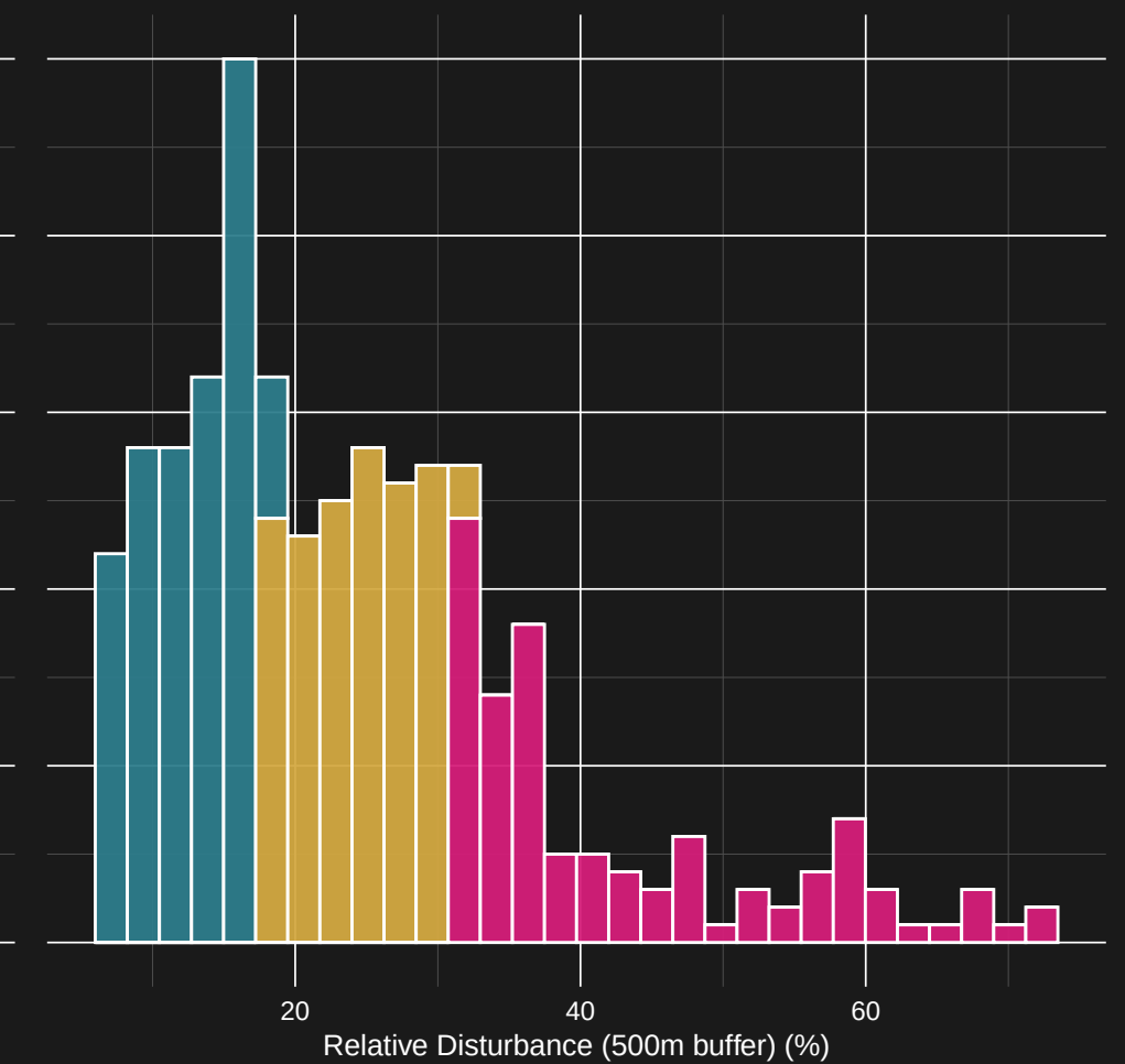
METHOD 3: Natural Breaks
