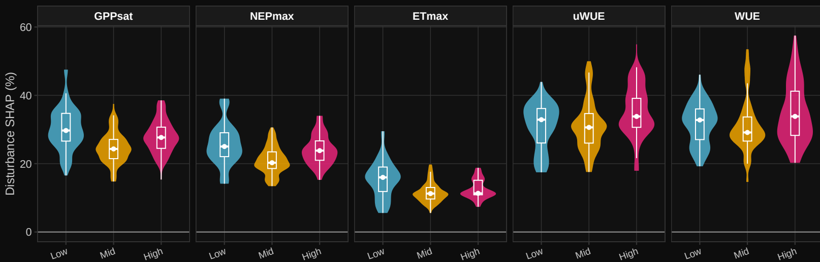
Disturbance SHAP % by Absolute Mortality (M8_anom 12m)
