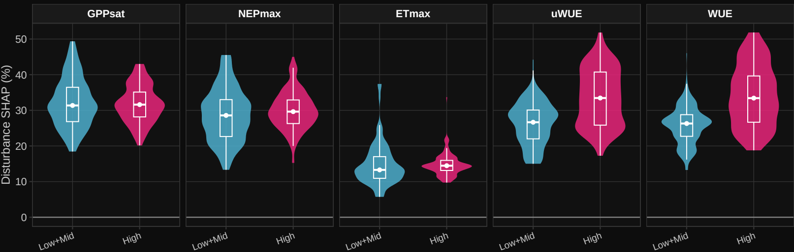
Disturbance SHAP % by Relative Disturbance (M6_raw 24m)
