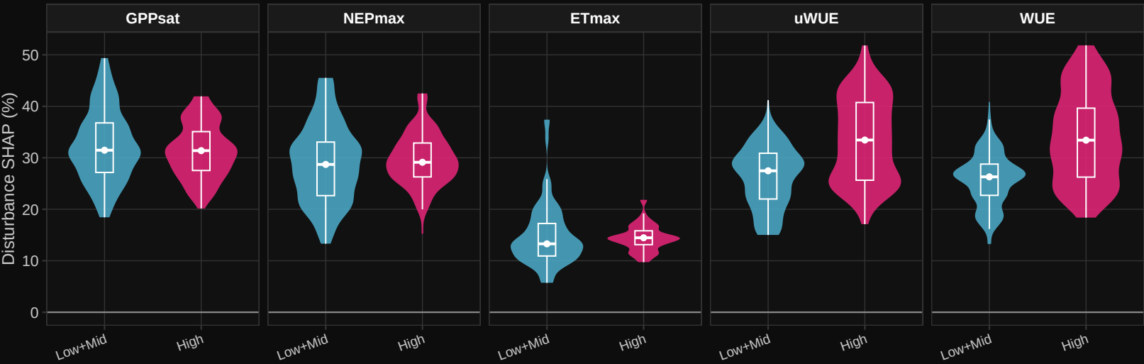
Disturbance SHAP % by Relative Mortality (M6_raw 24m)
