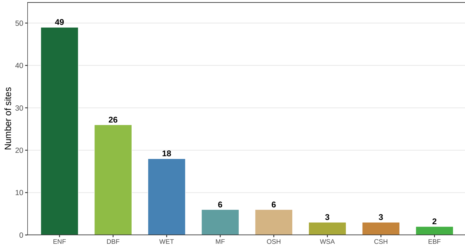
Sites per IGBP class – All sites (n = 113 total)
