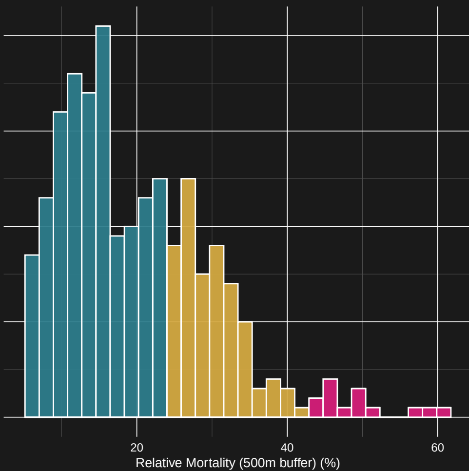
METHOD 2: Equal-Width
