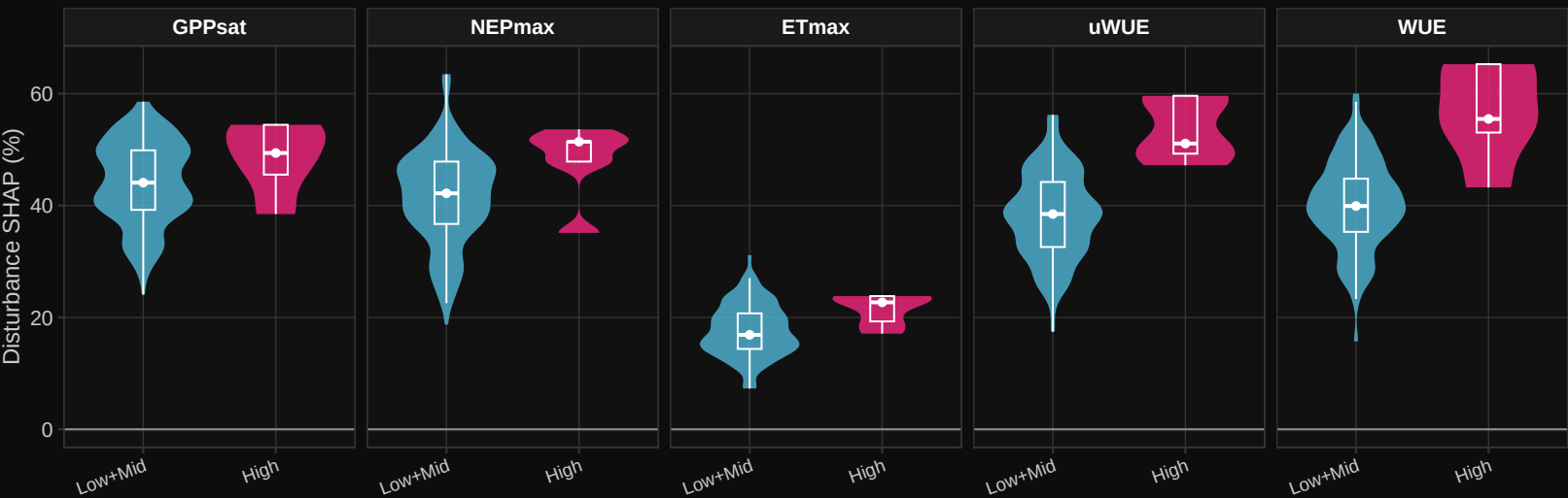
Disturbance SHAP % by Relative Disturbance (M6_anom 12m)
