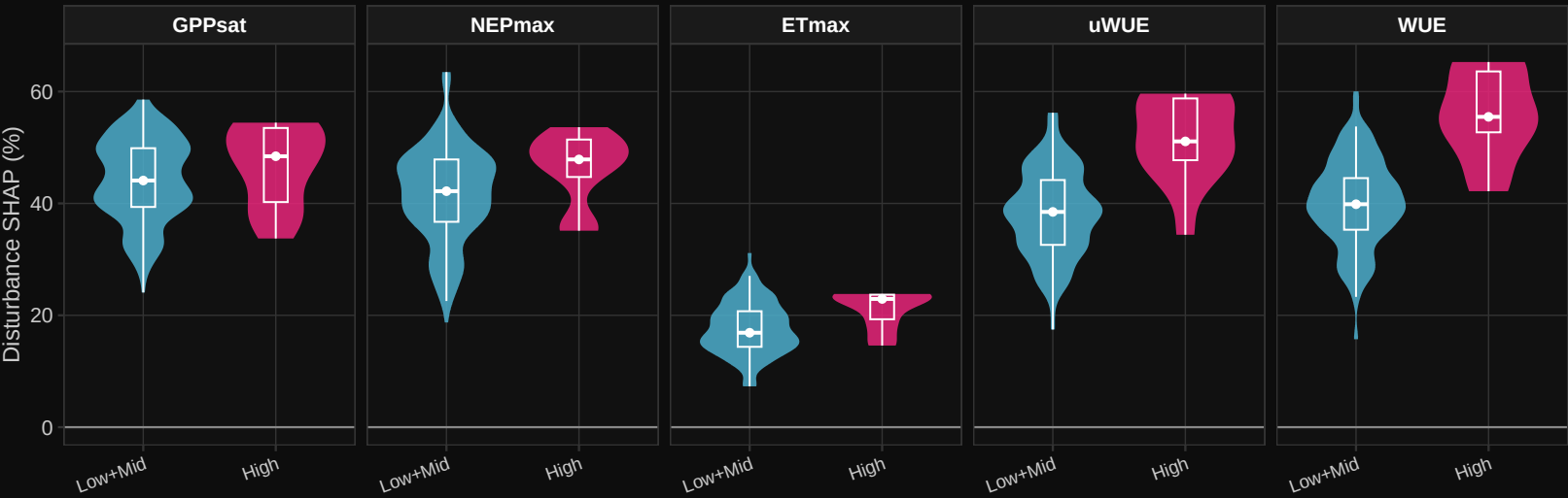
Disturbance SHAP % by Relative Mortality (M6_anom 12m)
