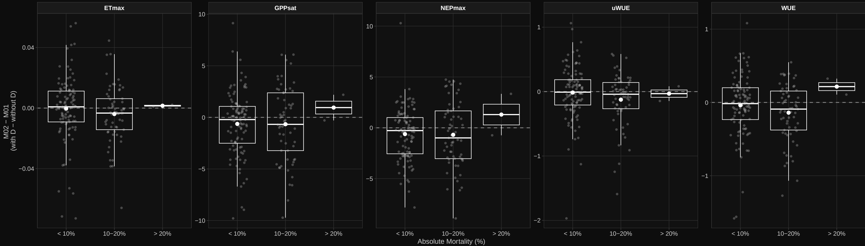
Delta RMSE vs Absolute Mortality – 12m
