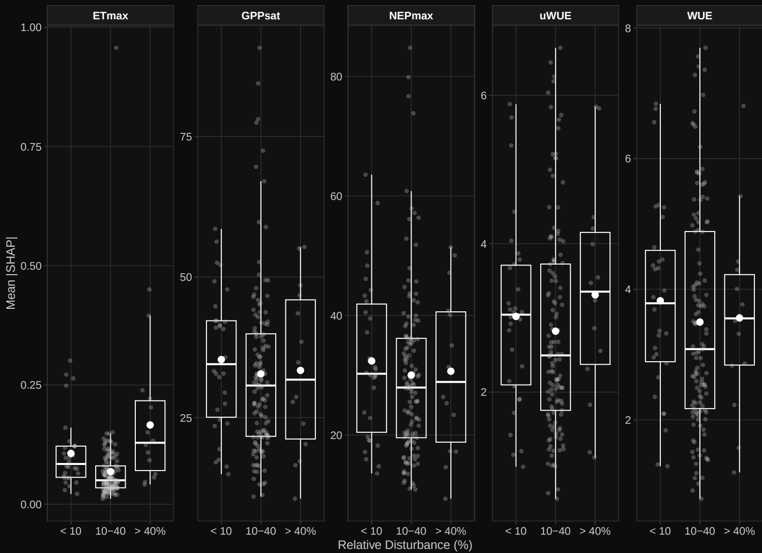
Disturbance SHAP vs Relative Disturbance – 24m
